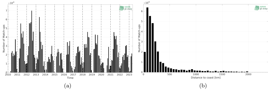
Figure 1: Number of match-ups between TSG (SAMOS) and SMOS SSS L2 v700 (ESA) SSS as a function of time (a) and as function of the distance to coast (b) over the North Atlantic Ocean Pi-MEP region and for the full satellite product period.
