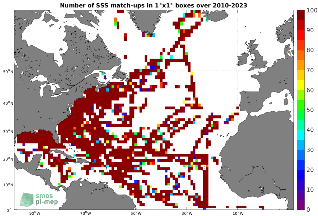
Figure 4: Number of SSS match-ups between TSG (SAMOS) SSS and the SMOS SSS L2 v700 (ESA) SSS product for the North Atlantic Ocean Pi-MEP region over 1^\circ \times 1^\circ boxes and for the full satellite product period.
