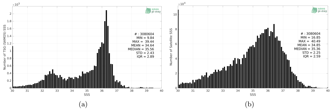
Figure 2: Histograms of SSS from TSG (SAMOS) (a) and SMOS SSS L2 v700 (ESA) (b) considering all match-up pairs per bins of 0.1 over the North Atlantic Ocean Pi-MEP region and for the full satellite product period.
