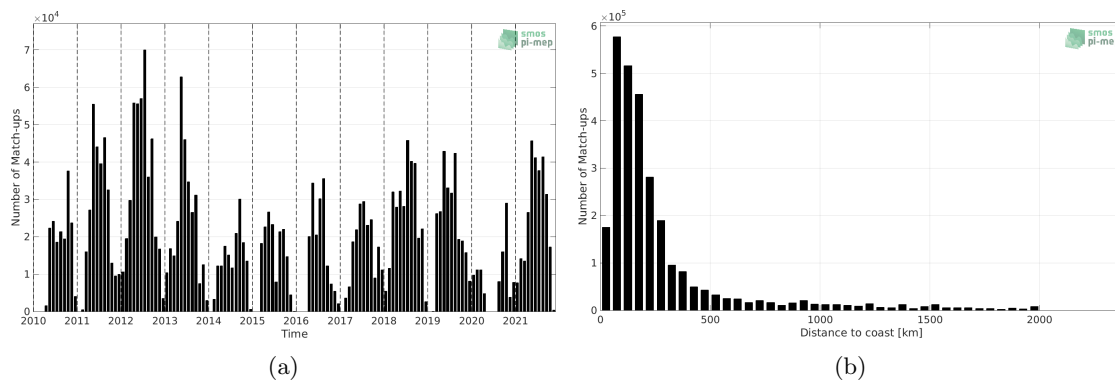
Figure 1: Number of match-ups between TSG (SAMOS) and SMOS SSS L2 v700 (ESA) SSS as a function of time (a) and as function of the distance to coast (b) over the North Atlantic Ocean Pi-MEP region and for the full satellite product period.
