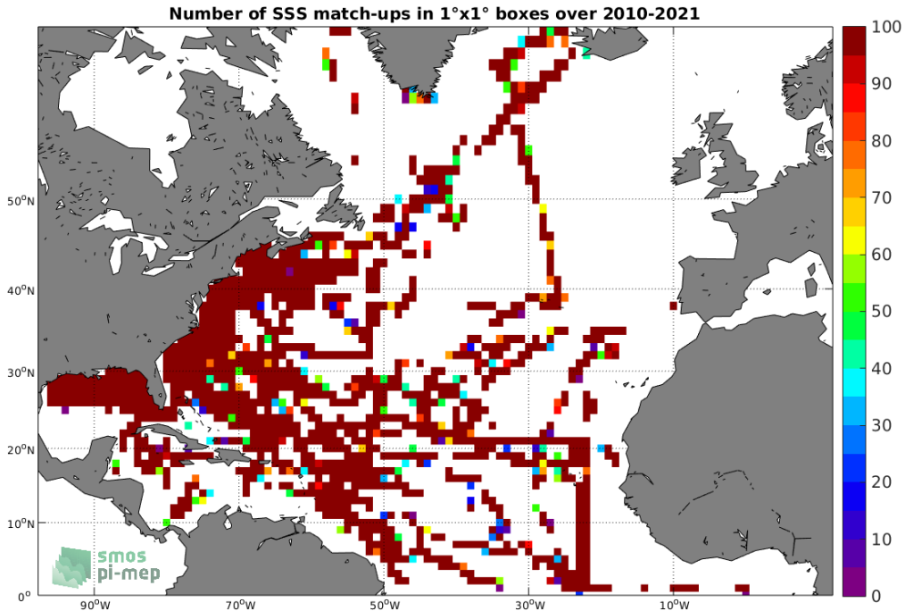
Figure 4: Number of SSS match-ups between TSG (SAMOS) SSS and the SMOS SSS L2 v700 (ESA) SSS product for the North Atlantic Ocean Pi-MEP region over 1°x1° boxes and for the full satellite product period.
