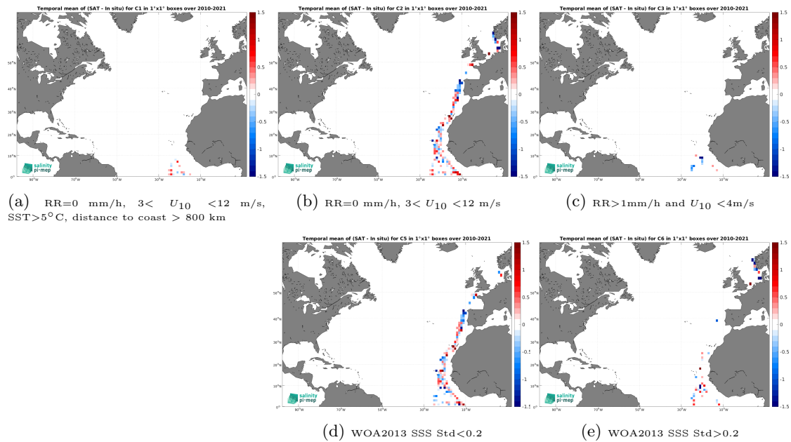
Figure 12: Temporal mean gridded over spatial boxes of size 1^\circ \times 1^\circ of \Delta\text{SSS} (SMOS SSS L2 v700 (ESA) - TSG (Polarstern)) for 5 different subdatasets corresponding to:RR=0 mm/h, 3 < U_{10} < 12 m/s, SST >5^\circ\text{C} , distance to coast > 800 km (a), RR=0 mm/h, 3 < U_{10} < 12 m/s (b), RR >1 mm/h and U_{10} < 4 m/s (c), WOA2013 SSS Std <0.2 (d), WOA2013 SSS Std >0.2 (e).
