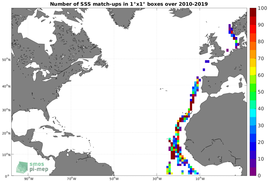
Figure 4: Number of SSS match-ups between TSG (Polarstern) SSS and the SMOS SSS L2 v700 (ESA) SSS product for the North Atlantic Ocean Pi-MEP region over 1°×1° boxes and for the full satellite product period.
