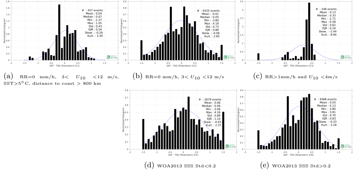
Figure 13: Normalized histogram of \Delta SSS (SMOS SSS L2 v700 (ESA) - TSG (Polarstern)) for 5 different subdatasets corresponding to: RR=0 mm/h, 3 < U_{10} < 12 m/s, SST>5°C, distance to coast > 800 km (a), RR=0 mm/h, 3 < U_{10} < 12 m/s (b), RR>1mm/h and U_{10} < 4 m/s (c), WOA2013 SSS Std<0.2 (d), WOA2013 SSS Std>0.2 (e).
