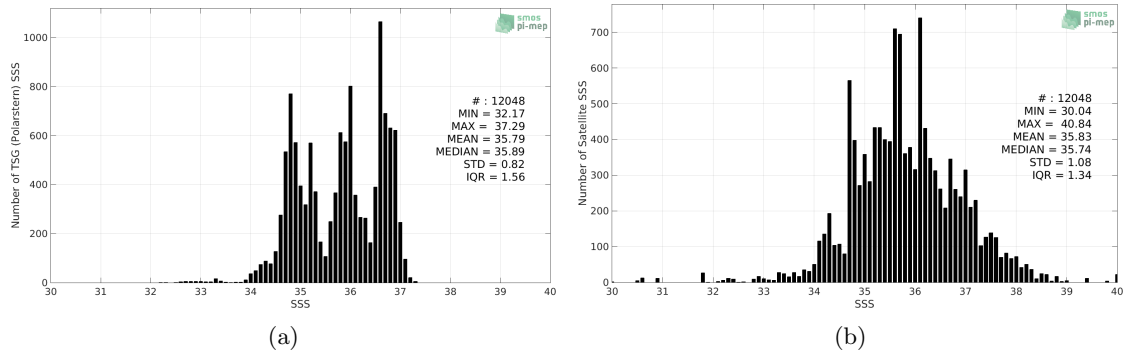
Figure 2: Histograms of SSS from TSG (Polarstern) (a) and SMOS SSS L2 v700 (ESA) (b) considering all match-up pairs per bins of 0.1 over the North Atlantic Ocean Pi-MEP region and for the full satellite product period.
