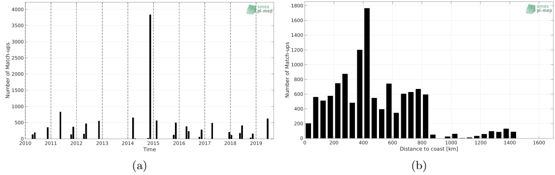
Figure 1: Number of match-ups between TSG (Polarstern) and SMOS SSS L2 v700 (ESA) SSS as a function of time (a) and as function of the distance to coast (b) over the North Atlantic Ocean Pi-MEP region and for the full satellite product period.
