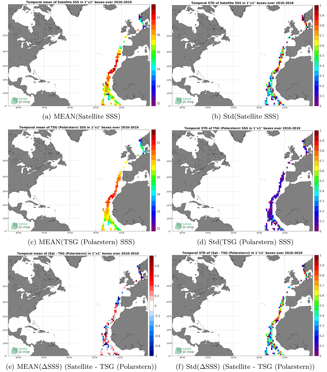
Figure 6: Temporal mean (left) and Std (right) of SSS from SMOS SSS L2 v700 (ESA) (top), TSG (Polarstern) (middle), and of \Delta SSS (Satellite - TSG (Polarstern)). Only match-up pairs are used to generate these maps.
