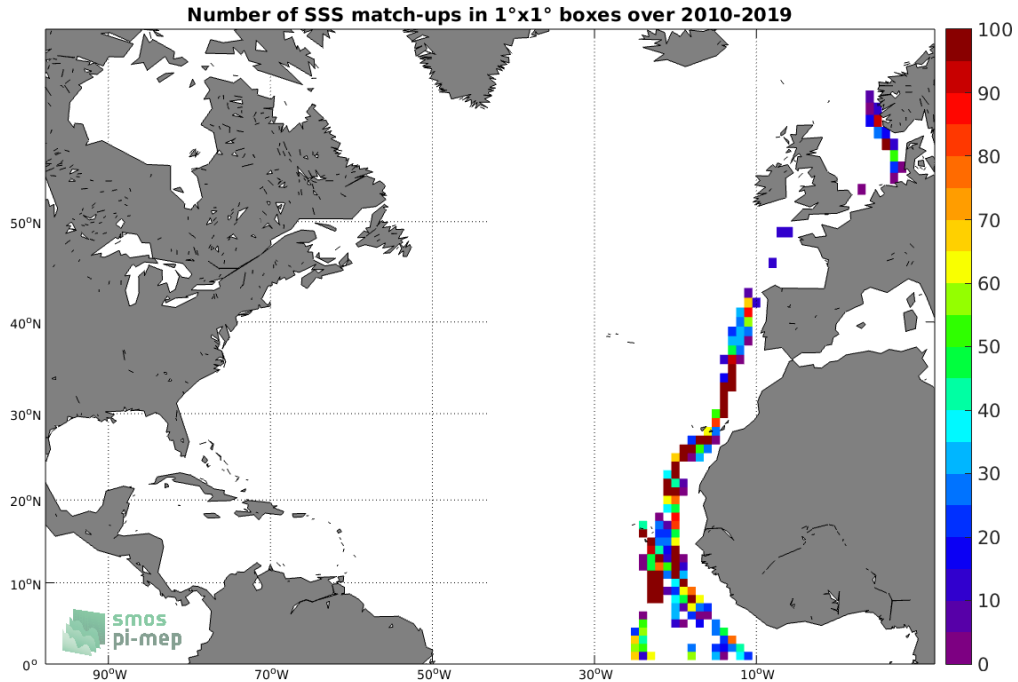
Figure 4: Number of SSS match-ups between TSG (Polarstern) SSS and the SMOS SSS L2 v700 (ESA) SSS product for the North Atlantic Ocean Pi-MEP region over 1^\circ \times 1^\circ boxes and for the full satellite product period.
