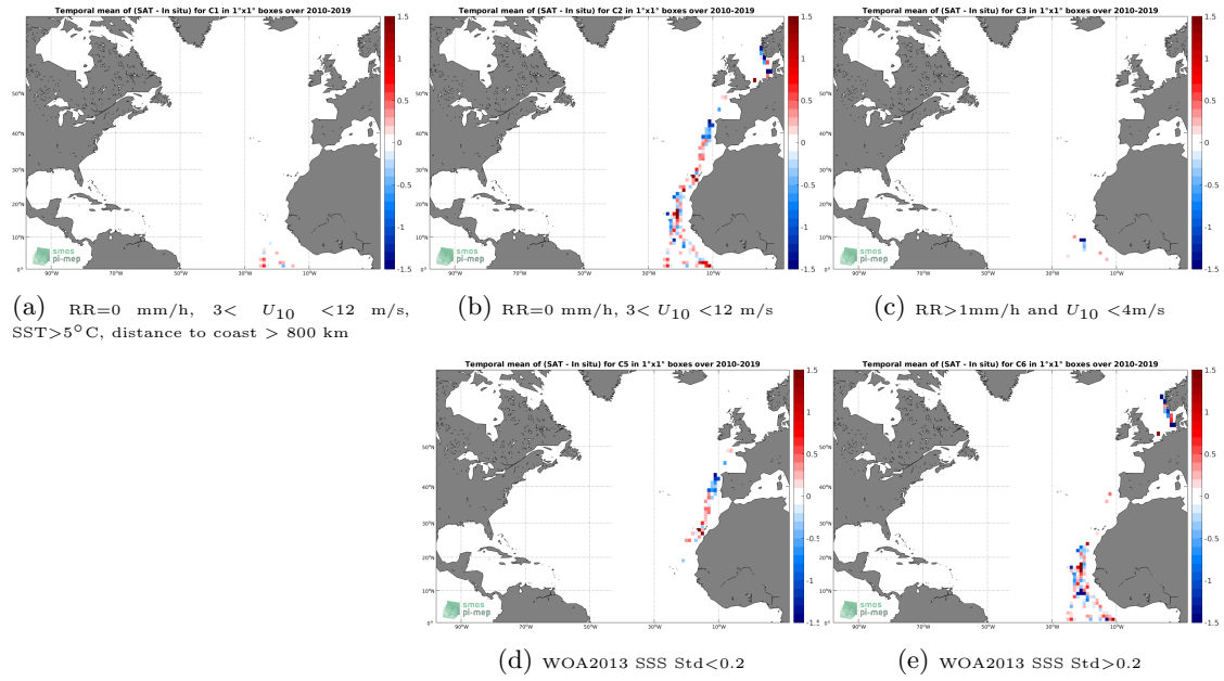
Figure 12: Temporal mean gridded over spatial boxes of size 1^\circ \times 1^\circ of \Delta SSS (SMOS SSS L2 v700 (ESA) - TSG (Polarstern)) for 5 different subdatasets corresponding to: RR=0 mm/h, 3 < U_{10} < 12 m/s, SST > 5^\circ\text{C} , distance to coast > 800 km (a), RR=0 mm/h, 3 < U_{10} < 12 m/s (b), RR > 1 mm/h and U_{10} < 4 m/s (c), WOA2013 SSS Std < 0.2 (d), WOA2013 SSS Std > 0.2 (e).
