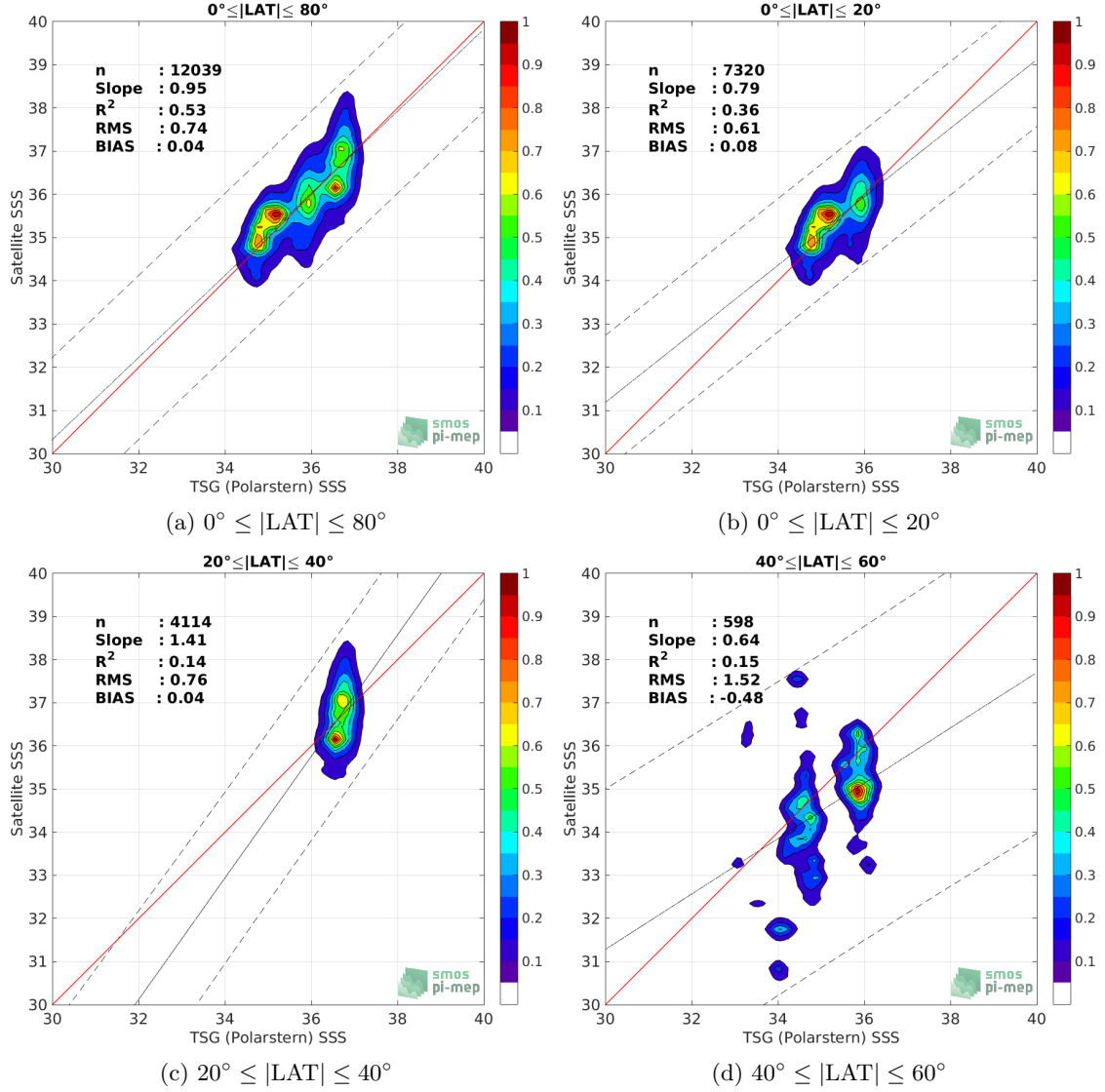
Figure 9: Contour maps of the concentration of SMOS SSS L2 v700 (ESA) SSS (y-axis) versus TSG (Polarstern) SSS (x-axis) at match-up pairs for different latitude bands. For each plot, the red line shows x=y . The black thin and dashed lines indicate a linear fit through the data cloud and the \pm 95\% confidence levels, respectively. The number match-up pairs n , the slope and R^2 coefficient of the linear fit, the root mean square (RMS) and the mean bias between satellite and in situ data are indicated for each latitude band in each plots.
