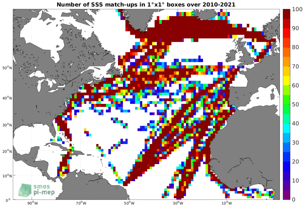
Figure 4: Number of SSS match-ups between TSG (LEGOS-DM) SSS and the SMOS SSS L2 v700 (ESA) SSS product for the North Atlantic Ocean Pi-MEP region over 1°x1° boxes and for the full satellite product period.
