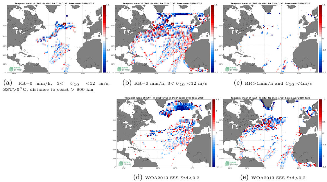
Figure 12: Temporal mean gridded over spatial boxes of size 1^\circ \times 1^\circ of \Delta\text{SSS} (SMOS SSS L2 v700 (ESA) - TSG (LEGOS-DM)) for 5 different subdatasets corresponding to:RR=0 mm/h, 3 < U_{10} < 12 m/s, SST >5^\circ\text{C} , distance to coast > 800 km (a), RR=0 mm/h, 3 < U_{10} < 12 m/s (b), RR >1 mm/h and U_{10} < 4 m/s (c), WOA2013 SSS Std <0.2 (d), WOA2013 SSS Std >0.2 (e).
