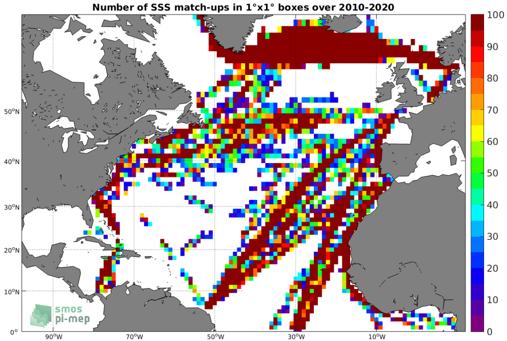
Figure 4: Number of SSS match-ups between TSG (LEGOS-DM) SSS and the SMOS SSS L2 v700 (ESA) SSS product for the North Atlantic Ocean Pi-MEP region over 1^{\circ} \times 1^{\circ} boxes and for the full satellite product period.
