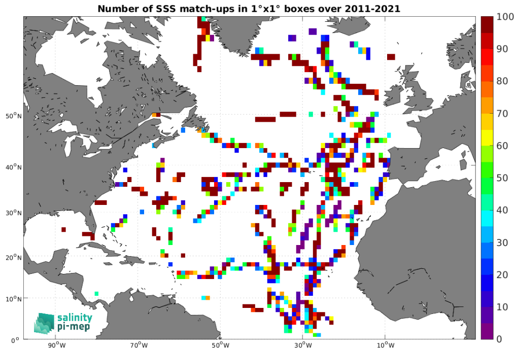
Figure 5: Number of SSS match-ups between TSG (GOSUD-Sailing-ship) SSS and the SMOS SSS L2 v700 (ESA) SSS product for the North Atlantic Ocean Pi-MEP region over 1^\circ \times 1^\circ boxes and for the full satellite product period.
