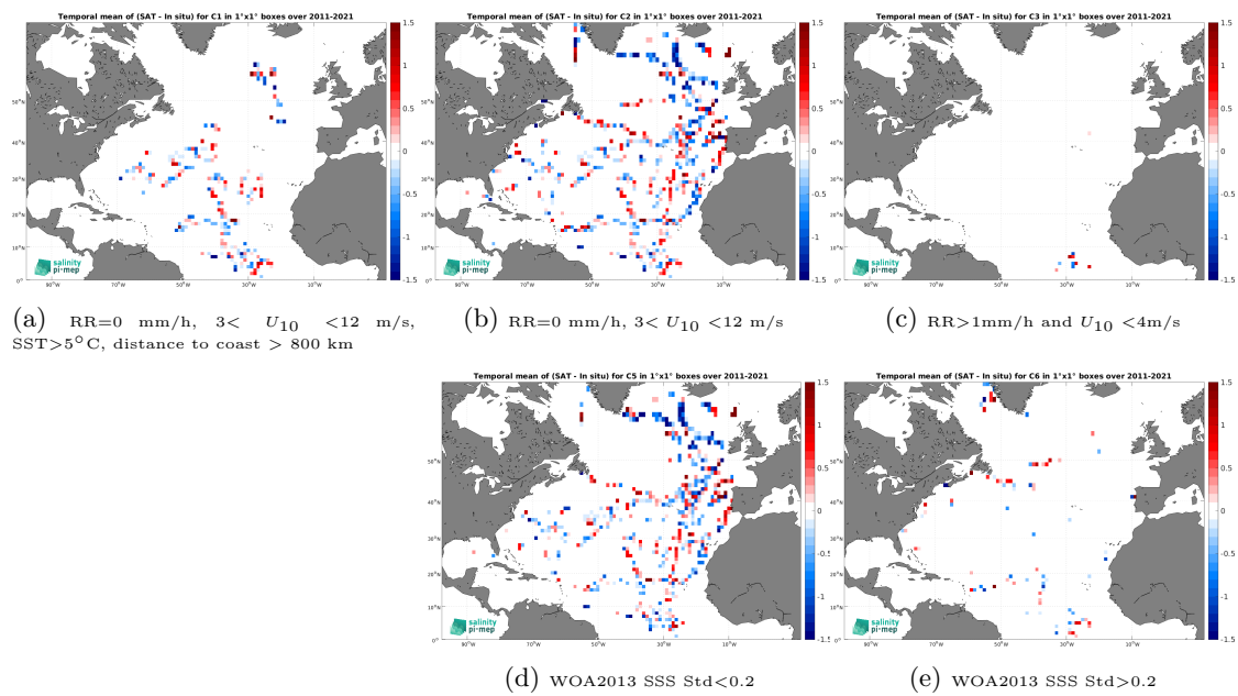
Figure 14: Temporal mean gridded over spatial boxes of size 1^\circ \times 1^\circ of \Delta\text{SSS} (SMOS SSS L2 v700 (ESA) - TSG (GOSUD-Sailing-ship)) for 5 different subdatasets corresponding to:RR=0 mm/h, 3 < U_{10} < 12 m/s, SST >5^\circ\text{C} , distance to coast > 800 km (a), RR=0 mm/h, 3 < U_{10} < 12 m/s (b), RR >1 mm/h and U_{10} < 4 m/s (c), WOA2013 SSS Std <0.2 (d), WOA2013 SSS Std >0.2 (e).
