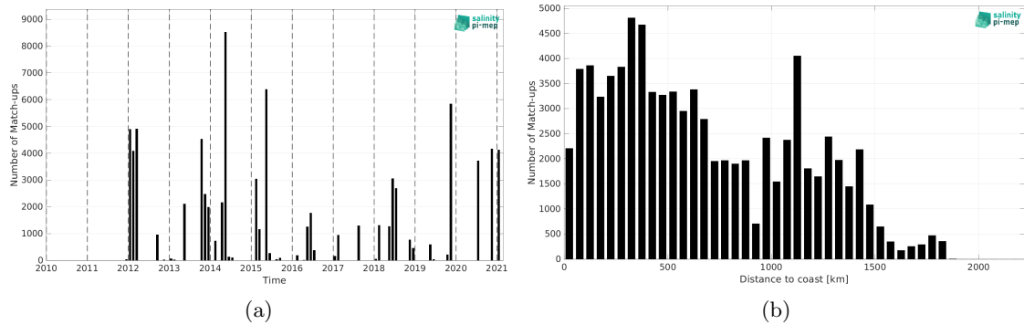
Figure 2: Number of match-ups between TSG (GOSUD-Sailing-ship) and SMOS SSS L2 v700 (ESA) SSS as a function of time (a) and as function of the distance to coast (b) over the North Atlantic Ocean Pi-MEP region and for the full satellite product period.
