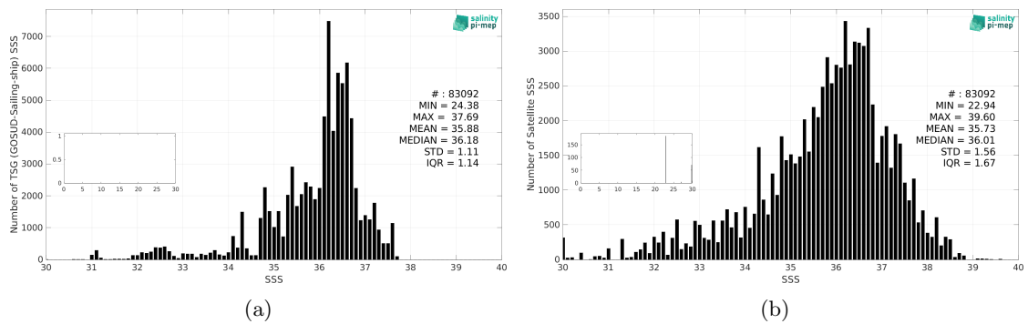
Figure 3: Histograms of SSS from TSG (GOSUD-Sailing-ship) (a) and SMOS SSS L2 v700 (ESA) (b) considering all match-up pairs per bins of 0.1 over the North Atlantic Ocean Pi-MEP region and for the full satellite product period.
