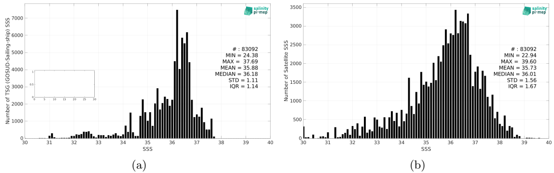
Figure 2: Histograms of SSS from TSG (GOSUD-Sailing-ship) (a) and SMOS SSS L2 v700 (ESA) (b) considering all match-up pairs per bins of 0.1 over the North Atlantic Ocean Pi-MEP region and for the full satellite product period.
