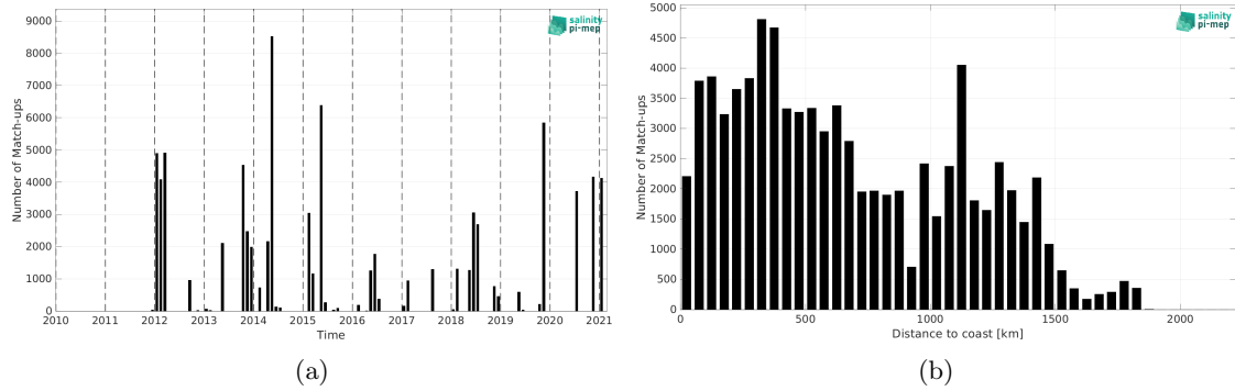
Figure 1: Number of match-ups between TSG (GOSUD-Sailing-ship) and SMOS SSS L2 v700 (ESA) SSS as a function of time (a) and as function of the distance to coast (b) over the North Atlantic Ocean Pi-MEP region and for the full satellite product period.
