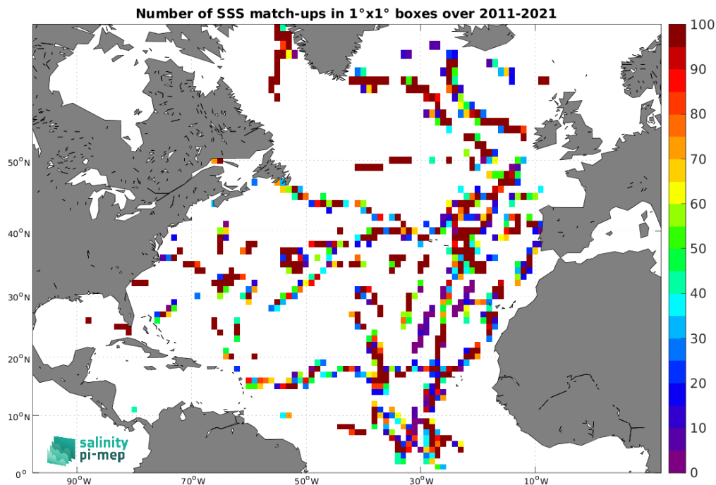
Figure 4: Number of SSS match-ups between TSG (GOSUD-Sailing-ship) SSS and the SMOS SSS L2 v700 (ESA) SSS product for the North Atlantic Ocean Pi-MEP region over 1^\circ \times 1^\circ boxes and for the full satellite product period.
