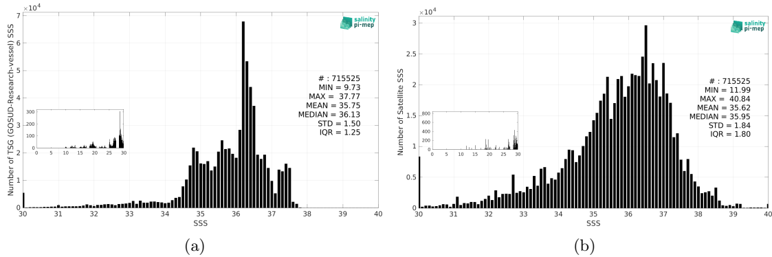
Figure 3: Histograms of SSS from TSG (GOSUD-Research-vessel) (a) and SMOS SSS L2 v700 (ESA) (b) considering all match-up pairs per bins of 0.1 over the North Atlantic Ocean Pi-MEP region and for the full satellite product period.
