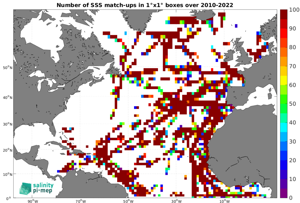
Figure 5: Number of SSS match-ups between TSG (GOSUD-Research-vessel) SSS and the SMOS SSS L2 v700 (ESA) SSS product for the North Atlantic Ocean Pi-MEP region over 1°x1° boxes and for the full satellite product period.
