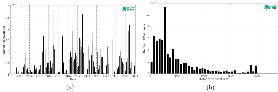
Figure 2: Number of match-ups between TSG (GOSUD-Research-vessel) and SMOS SSS L2 v700 (ESA) SSS as a function of time (a) and as function of the distance to coast (b) over the North Atlantic Ocean Pi-MEP region and for the full satellite product period.
