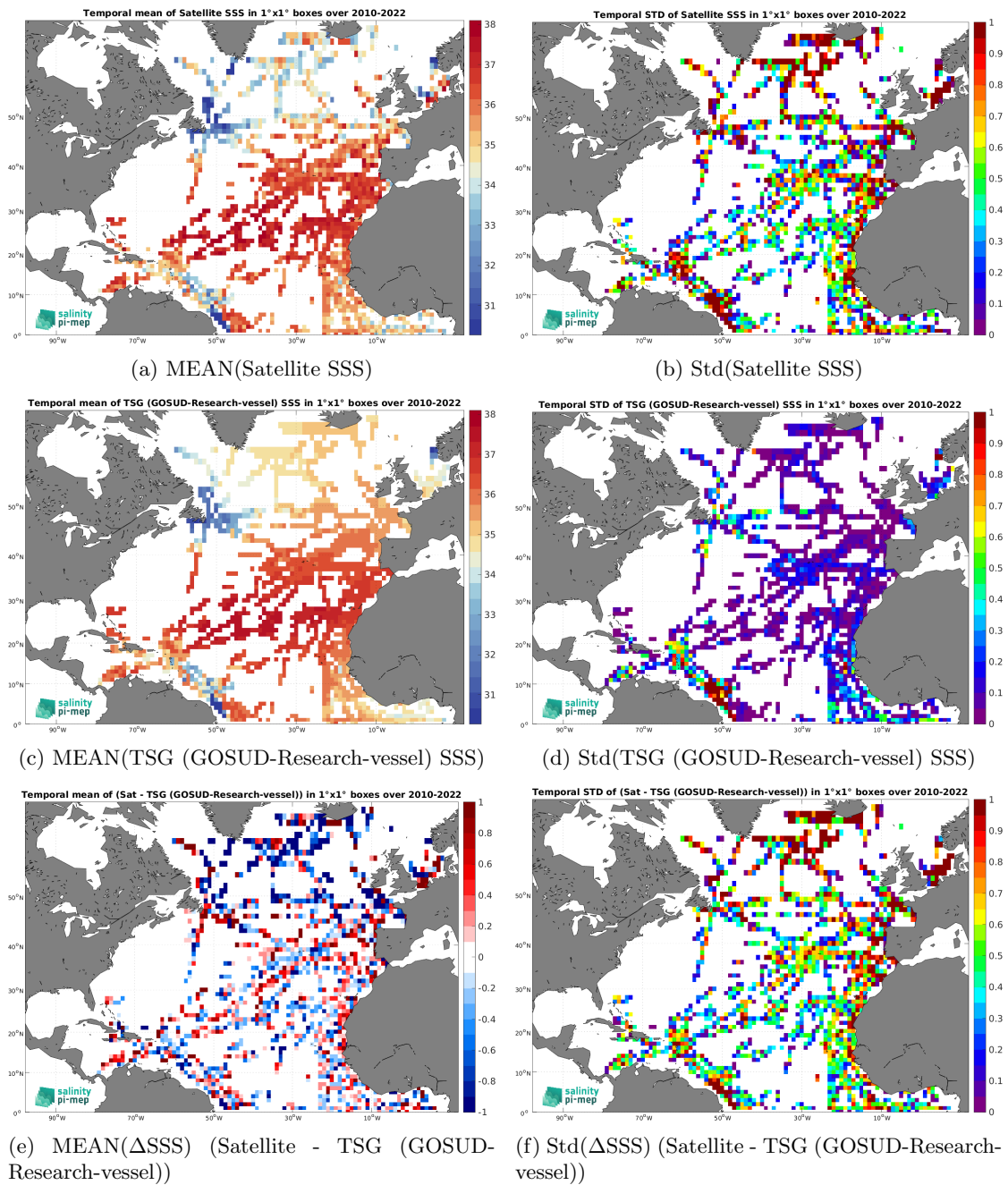
Figure 7: Temporal mean (left) and Std (right) of SSS from SMOS SSS L2 v700 (ESA) (top), TSG (GOSUD-Research-vessel) (middle), and of \Delta SSS (Satellite - TSG (GOSUD-Research-vessel)). Only match-up pairs are used to generate these maps.
