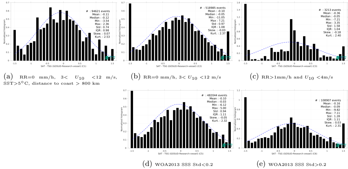
Figure 15: Normalized histogram of \Delta SSS (SMOS SSS L2 v700 (ESA) - TSG (GOSUD-Research-vessel)) for 5 different subdatasets corresponding to: RR=0 mm/h, 3 < U_{10} < 12 m/s, SST >5^{\circ} C, distance to coast > 800 km (a), RR=0 mm/h, 3 < U_{10} < 12 m/s (b), RR >1 mm/h and U_{10} < 4 m/s (c), WOA2013 SSS Std <0.2 (d), WOA2013 SSS Std >0.2 (e).
