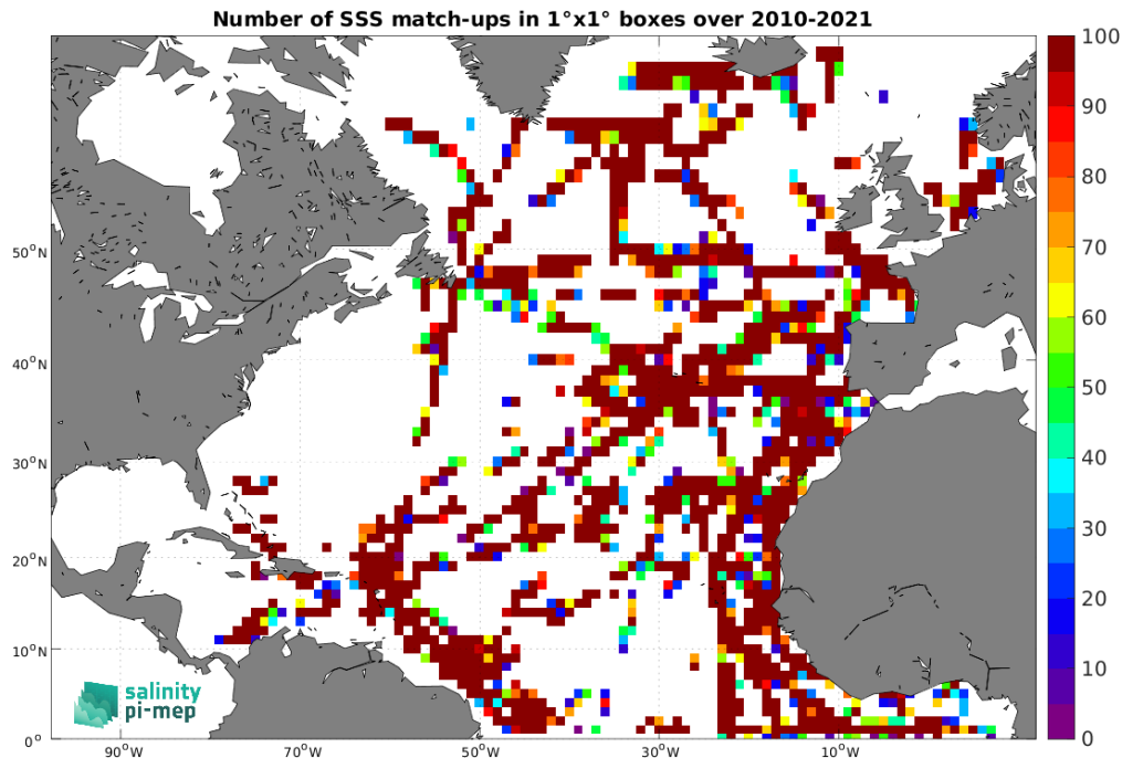
Figure 5: Number of SSS match-ups between TSG (GOSUD-Research-vessel) SSS and the SMOS SSS L2 v700 (ESA) SSS product for the North Atlantic Ocean Pi-MEP region over 1^\circ \times 1^\circ boxes and for the full satellite product period.
