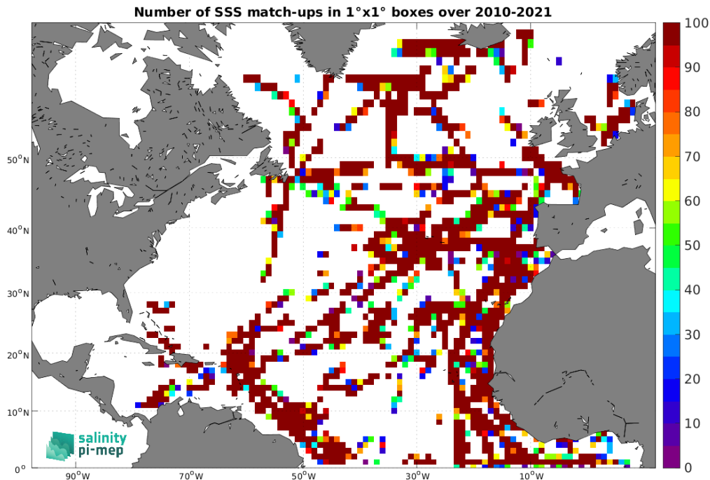
Figure 4: Number of SSS match-ups between TSG (GOSUD-Research-vessel) SSS and the SMOS SSS L2 v700 (ESA) SSS product for the North Atlantic Ocean Pi-MEP region over 1^\circ \times 1^\circ boxes and for the full satellite product period.
