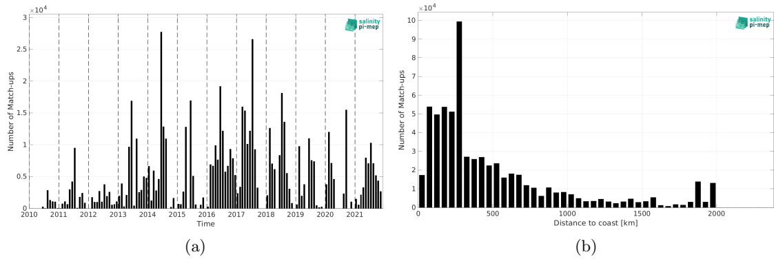
Figure 1: Number of match-ups between TSG (GOSUD-Research-vessel) and SMOS SSS L2 v700 (ESA) SSS as a function of time (a) and as function of the distance to coast (b) over the North Atlantic Ocean Pi-MEP region and for the full satellite product period.
