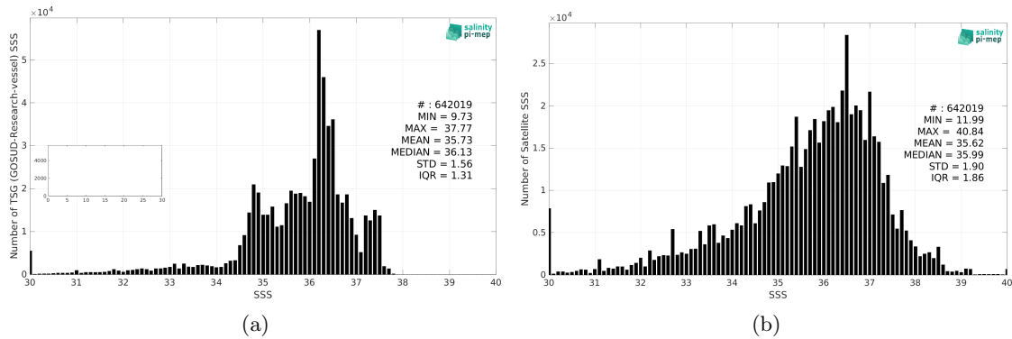
Figure 2: Histograms of SSS from TSG (GOSUD-Research-vessel) (a) and SMOS SSS L2 v700 (ESA) (b) considering all match-up pairs per bins of 0.1 over the North Atlantic Ocean Pi-MEP region and for the full satellite product period.
