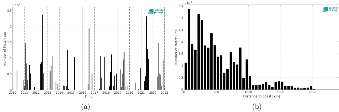
Figure 2: Number of match-ups between TSG (CSIC-UTM) and SMOS SSS L2 v700 (ESA) SSS as a function of time (a) and as function of the distance to coast (b) over the North Atlantic Ocean Pi-MEP region and for the full satellite product period.
