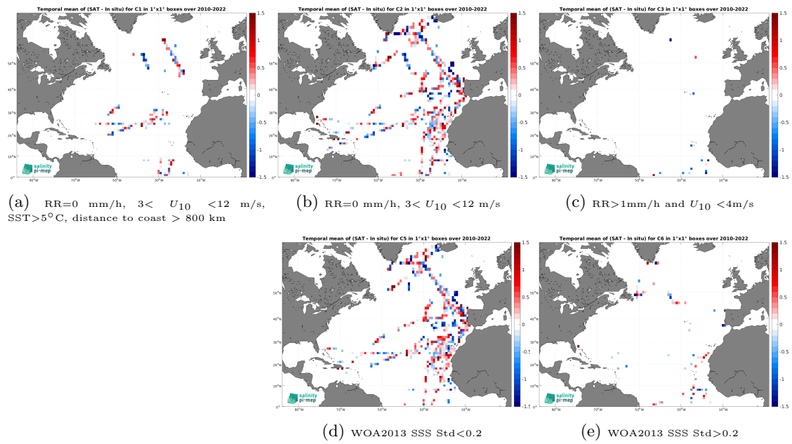
Figure 14: Temporal mean gridded over spatial boxes of size 1^\circ \times 1^\circ of \Delta SSS (SMOS SSS L2 v700 (ESA) - TSG (CSIC-UTM)) for 5 different subdatasets corresponding to:RR=0 mm/h, 3 < U_{10} < 12 m/s, SST>5°C, distance to coast > 800 km (a), RR=0 mm/h, 3 < U_{10} < 12 m/s (b), RR>1mm/h and U_{10} < 4 m/s (c), WOA2013 SSS Std<0.2 (d), WOA2013 SSS Std>0.2 (e).
