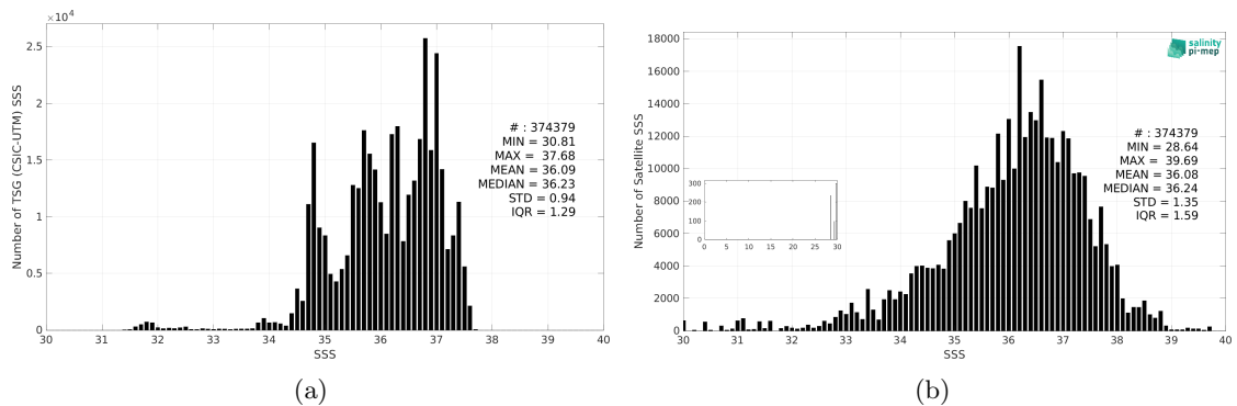
Figure 3: Histograms of SSS from TSG (CSIC-UTM) (a) and SMOS SSS L2 v700 (ESA) (b) considering all match-up pairs per bins of 0.1 over the North Atlantic Ocean Pi-MEP region and for the full satellite product period.
