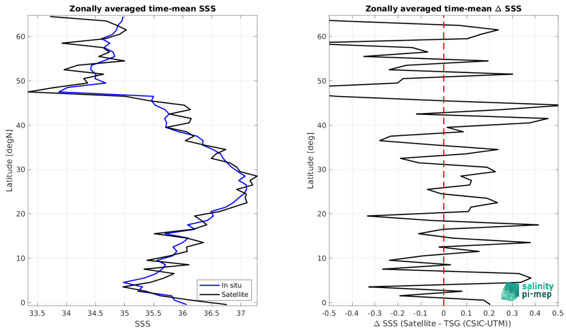
Figure 9: Left panel: Zonal mean SSS from SMOS SSS L2 v700 (ESA) satellite product (black) and from TSG (CSIC-UTM) (blue). Right panel: Zonal mean of \Delta SSS (Satellite - TSG (CSIC-UTM)) for all the collected Pi-MEP match-up pairs estimated over the full satellite product period.
