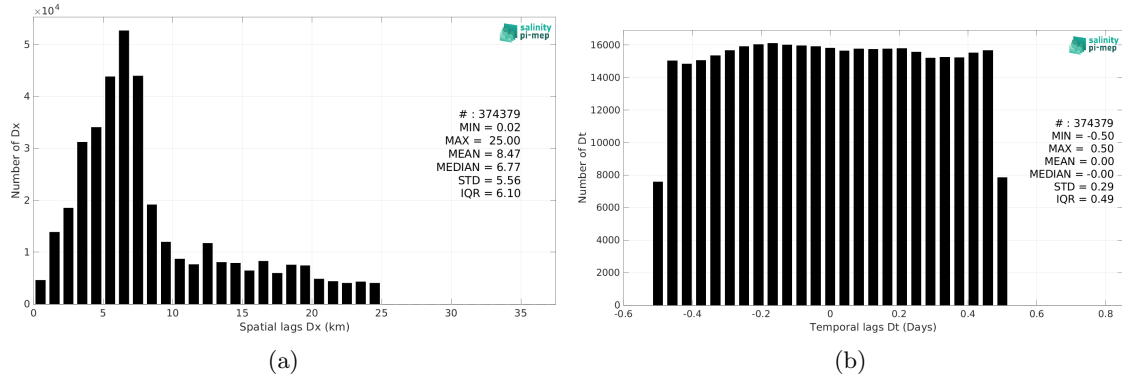
Figure 6: Histograms of the spatial (a) and temporal (b) lags between the location/time of the TSG (CSIC-UTM) measurement and the date of the corresponding SMOS SSS L2 v700 (ESA) SSS pixel.
