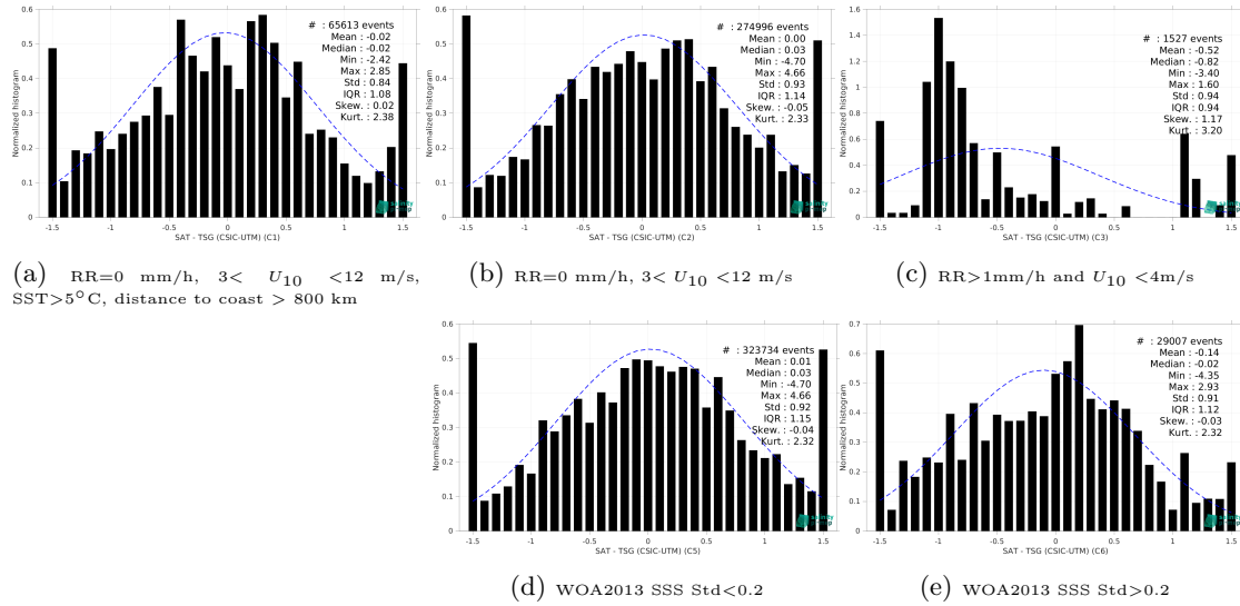
Figure 15: Normalized histogram of \Delta SSS (SMOS SSS L2 v700 (ESA) - TSG (CSIC-UTM)) for 5 different subdatasets corresponding to: RR=0 mm/h, 3 < U_{10} < 12 m/s, SST>5°C, distance to coast > 800 km (a), RR=0 mm/h, 3 < U_{10} < 12 m/s (b), RR>1mm/h and U_{10} < 4 m/s (c), WOA2013 SSS Std<0.2 (d), WOA2013 SSS Std>0.2 (e).
