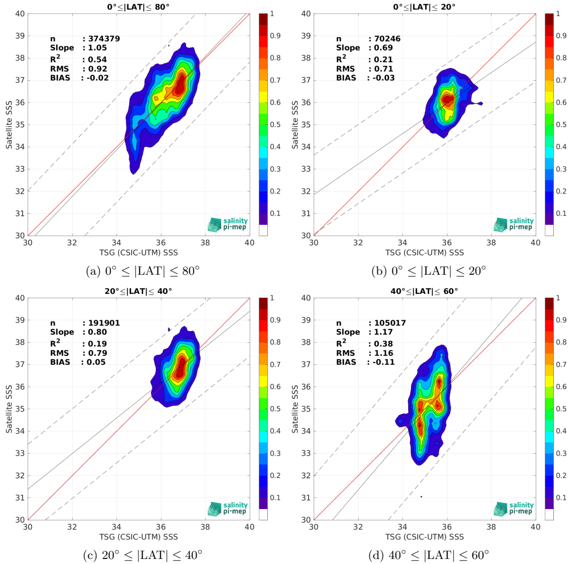
Figure 10: Contour maps of the concentration of SMOS SSS L2 v700 (ESA) SSS (y-axis) versus TSG (CSIC-UTM) SSS (x-axis) at match-up pairs for different latitude bands. For each plot, the red line shows x=y . The black thin and dashed lines indicate a linear fit through the data cloud and the \pm 95\% confidence levels, respectively. The number match-up pairs n , the slope and R^2 coefficient of the linear fit, the root mean square (RMS) and the mean bias between satellite and in situ data are indicated for each latitude band in each plots.
