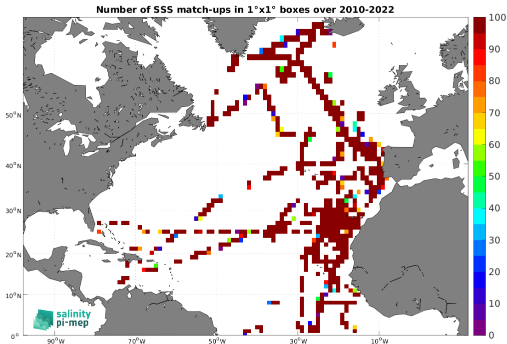
Figure 5: Number of SSS match-ups between TSG (CSIC-UTM) SSS and the SMOS SSS L2 v700 (ESA) SSS product for the North Atlantic Ocean Pi-MEP region over 1^\circ \times 1^\circ boxes and for the full satellite product period.
