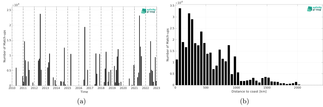
Figure 1: Number of match-ups between TSG (CSIC-UTM) and SMOS SSS L2 v700 (ESA) SSS as a function of time (a) and as function of the distance to coast (b) over the North Atlantic Ocean Pi-MEP region and for the full satellite product period.
