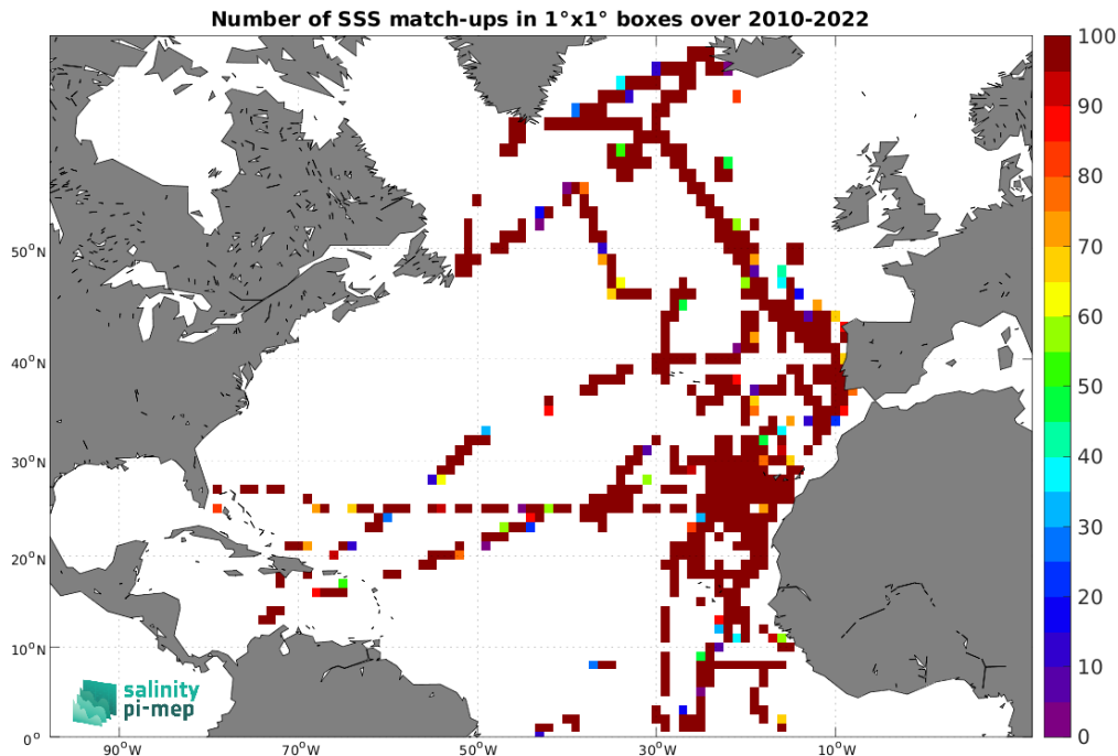
Figure 4: Number of SSS match-ups between TSG (CSIC-UTM) SSS and the SMOS SSS L2 v700 (ESA) SSS product for the North Atlantic Ocean Pi-MEP region over 1^\circ \times 1^\circ boxes and for the full satellite product period.
