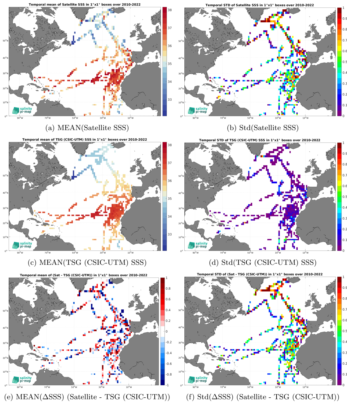
Figure 6: Temporal mean (left) and Std (right) of SSS from SMOS SSS L2 v700 (ESA) (top), TSG (CSIC-UTM) (middle), and of \Delta SSS (Satellite - TSG (CSIC-UTM)). Only match-up pairs are used to generate these maps.
