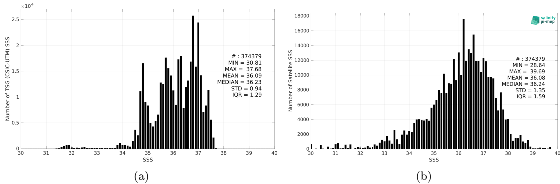
Figure 2: Histograms of SSS from TSG (CSIC-UTM) (a) and SMOS SSS L2 v700 (ESA) (b) considering all match-up pairs per bins of 0.1 over the North Atlantic Ocean Pi-MEP region and for the full satellite product period.
