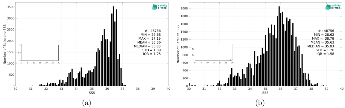
Figure 3: Histograms of SSS from Sairdrone (a) and SMOS SSS L2 v700 (ESA) (b) considering all match-up pairs per bins of 0.1 over the North Atlantic Ocean Pi-MEP region and for the full satellite product period.
