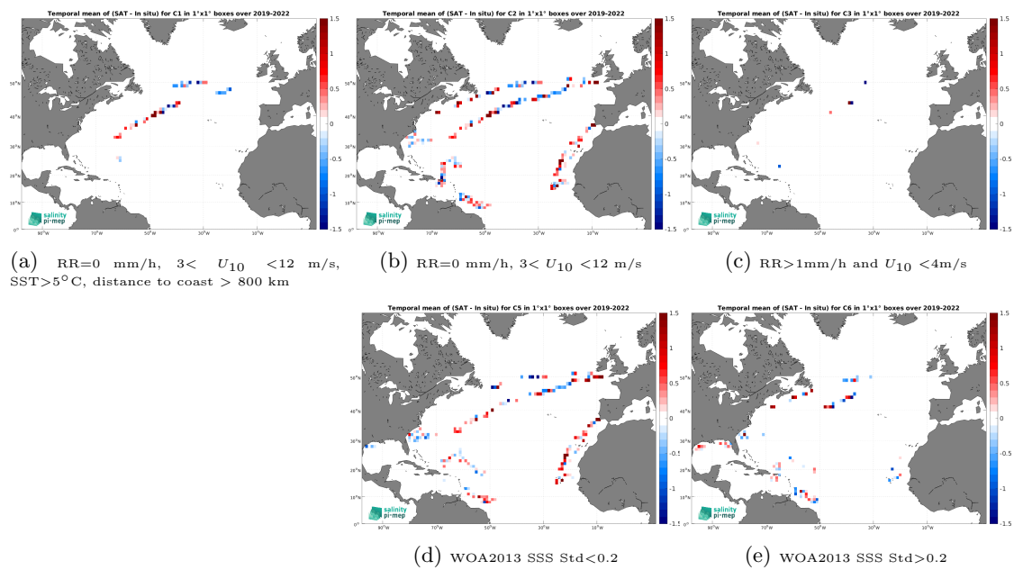
Figure 14: Temporal mean gridded over spatial boxes of size 1^\circ \times 1^\circ of \Delta\text{SSS} (SMOS SSS L2 v700 (ESA) - Saifdrone) for 5 different subdatasets corresponding to: RR=0 mm/h, 3 < U_{10} < 12 m/s, SST > 5°C, distance to coast > 800 km (a), RR=0 mm/h, 3 < U_{10} < 12 m/s (b), RR > 1mm/h and U_{10} < 4 m/s (c), WOA2013 SSS Std < 0.2 (d), WOA2013 SSS Std > 0.2 (e).
