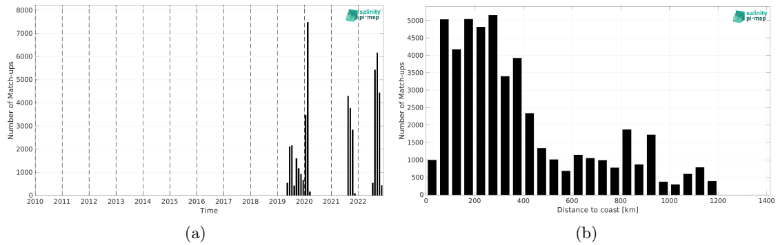
Figure 2: Number of match-ups between Sairdrone and SMOS SSS L2 v700 (ESA) SSS as a function of time (a) and as function of the distance to coast (b) over the North Atlantic Ocean Pi-MEP region and for the full satellite product period.
