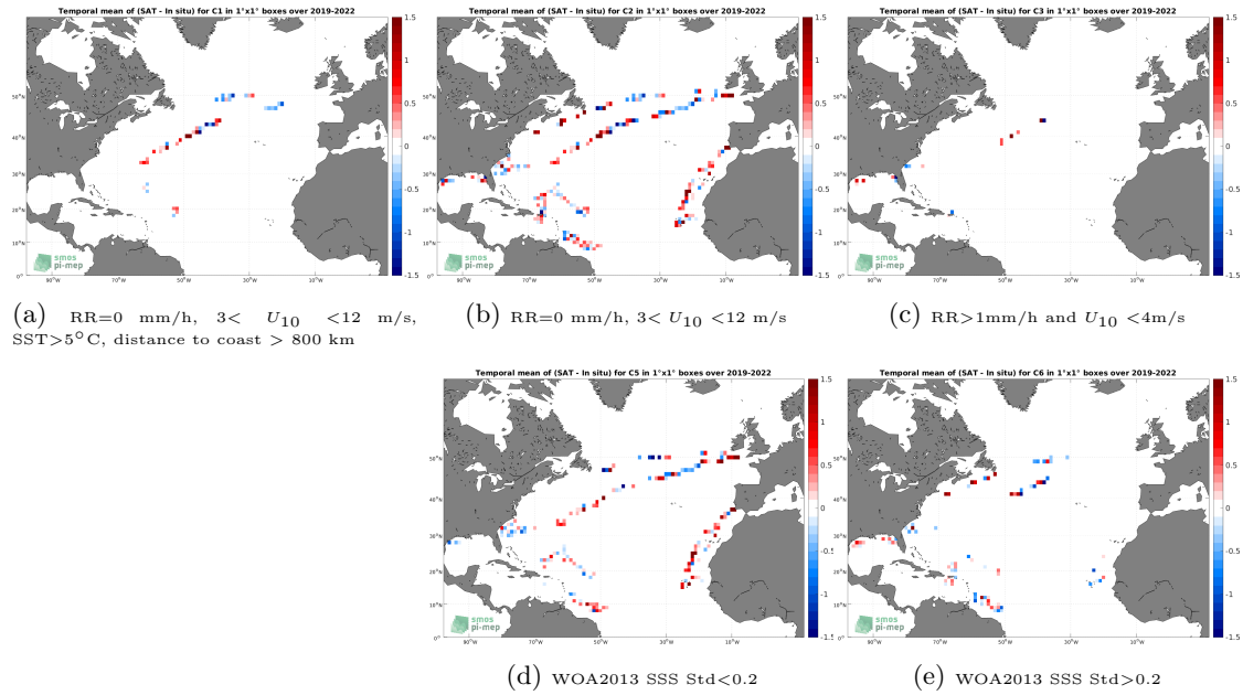
Figure 12: Temporal mean gridded over spatial boxes of size 1^\circ \times 1^\circ of \Delta\text{SSS} (SMOS SSS L2 v700 (ESA) - Sairdrone) for 5 different subdatasets corresponding to:RR=0 mm/h, 3 < U_{10} < 12 m/s, SST >5^\circ\text{C} , distance to coast > 800 km (a), RR=0 mm/h, 3 < U_{10} < 12 m/s (b), RR >1 mm/h and U_{10} < 4 m/s (c), WOA2013 SSS Std <0.2 (d), WOA2013 SSS Std >0.2 (e).
