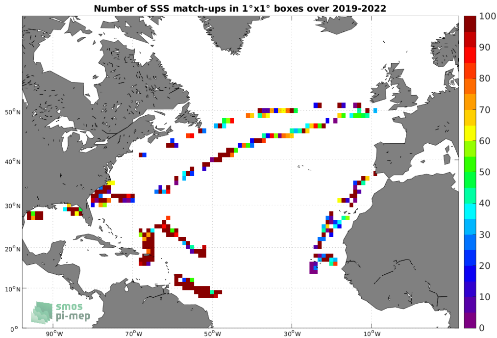
Figure 4: Number of SSS match-ups between Saildrone SSS and the SMOS SSS L2 v700 (ESA) SSS product for the North Atlantic Ocean Pi-MEP region over 1^\circ \times 1^\circ boxes and for the full satellite product period.
