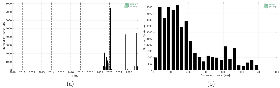
Figure 1: Number of match-ups between Sairdrone and SMOS SSS L2 v700 (ESA) SSS as a function of time (a) and as function of the distance to coast (b) over the North Atlantic Ocean Pi-MEP region and for the full satellite product period.
