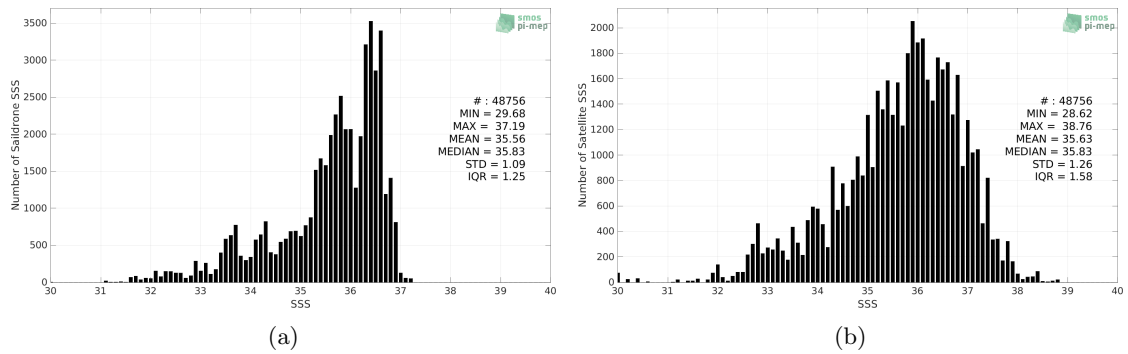
Figure 2: Histograms of SSS from Sairdrone (a) and SMOS SSS L2 v700 (ESA) (b) considering all match-up pairs per bins of 0.1 over the North Atlantic Ocean Pi-MEP region and for the full satellite product period.
