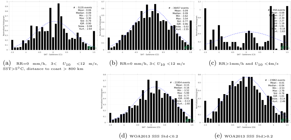
Figure 13: Normalized histogram of \Delta SSS (SMOS SSS L2 v700 (ESA) - Saildrone) for 5 different subdatasets corresponding to: RR=0 mm/h, 3 < U_{10} < 12 m/s, SST > 5°C, distance to coast > 800 km (a), RR=0 mm/h, 3 < U_{10} < 12 m/s (b), RR > 1mm/h and U_{10} < 4 m/s (c), WOA2013 SSS Std < 0.2 (d), WOA2013 SSS Std > 0.2 (e).
