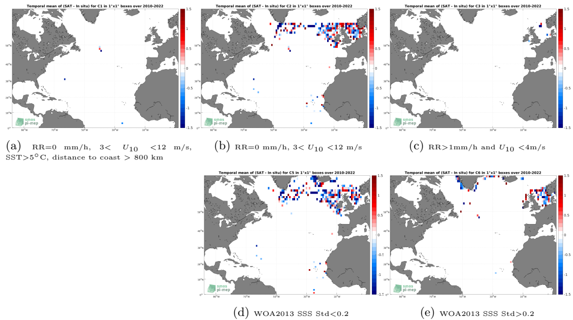
Figure 12: Temporal mean gridded over spatial boxes of size 1^\circ \times 1^\circ of \Delta SSS (SMOS SSS L2 v700 (ESA) - ICES) for 5 different subdatasets corresponding to:RR=0 mm/h, 3 < U_{10} < 12 m/s, SST >5^\circ C, distance to coast > 800 km (a), RR=0 mm/h, 3 < U_{10} < 12 m/s (b), RR >1 mm/h and U_{10} < 4 m/s (c), WOA2013 SSS Std <0.2 (d), WOA2013 SSS Std >0.2 (e).
