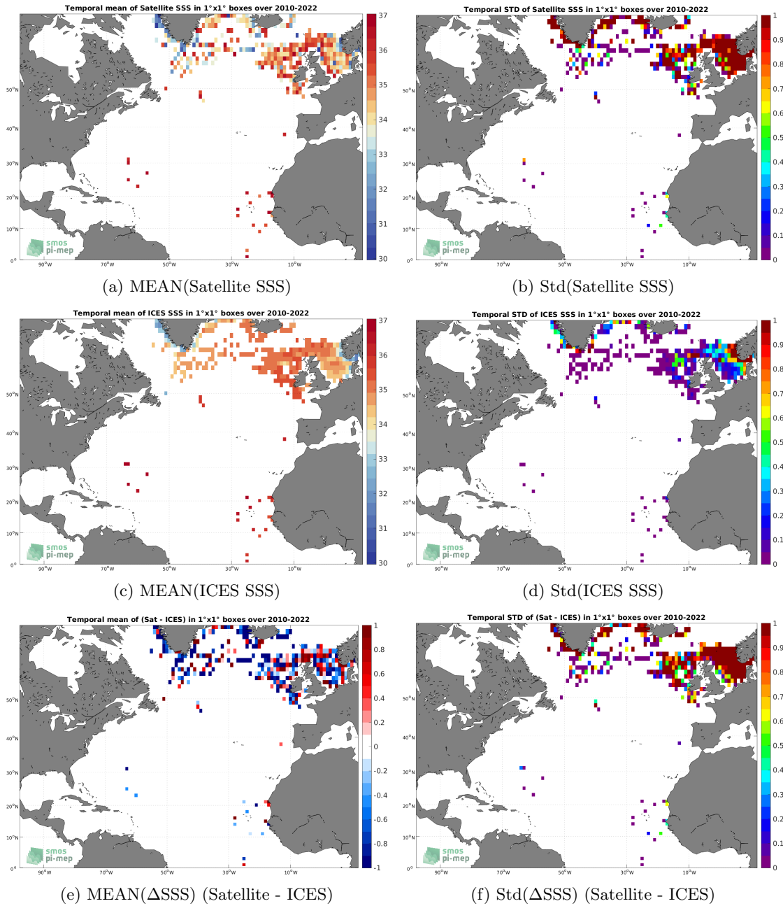
Figure 6: Temporal mean (left) and Std (right) of SSS from SMOS SSS L2 v700 (ESA) (top), ICES (middle), and of \Delta SSS (Satellite - ICES). Only match-up pairs are used to generate these maps.
