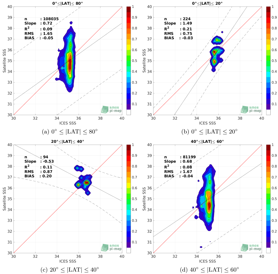
Figure 9: Contour maps of the concentration of SMOS SSS L2 v700 (ESA) SSS (y-axis) versus ICES SSS (x-axis) at match-up pairs for different latitude bands. For each plot, the red line shows x=y . The black thin and dashed lines indicate a linear fit through the data cloud and the \pm 95\% confidence levels, respectively. The number match-up pairs n , the slope and R^2 coefficient of the linear fit, the root mean square (RMS) and the mean bias between satellite and in situ data are indicated for each latitude band in each plots.
