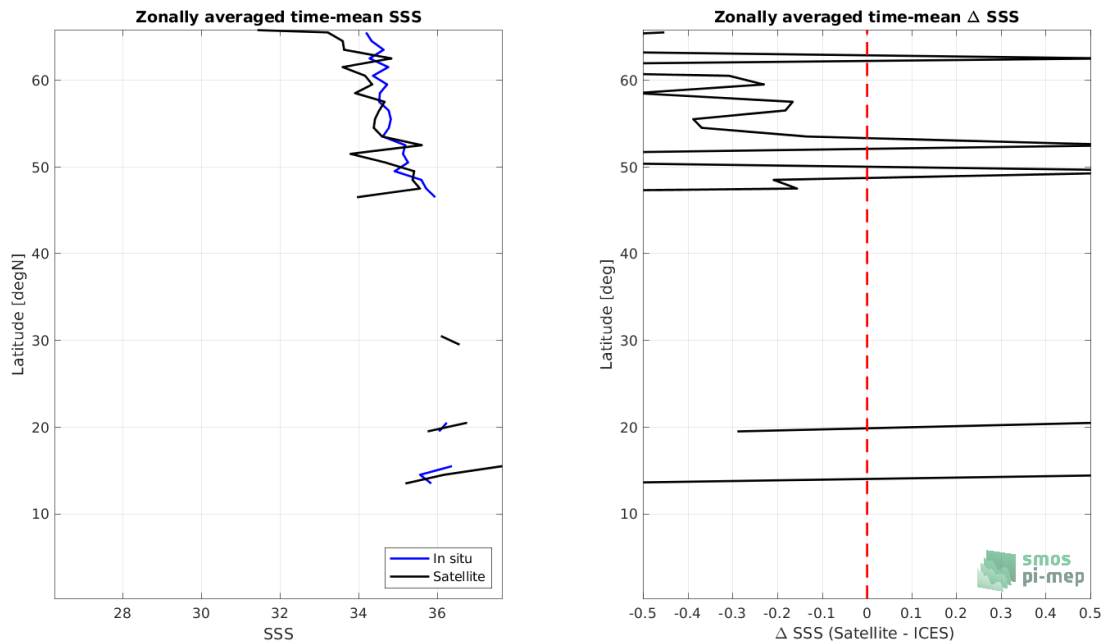
Figure 8: Left panel: Zonal mean SSS from SMOS SSS L2 v700 (ESA) satellite product (black) and from ICES (blue). Right panel: Zonal mean of \Delta SSS (Satellite - ICES) for all the collected Pi-MEP match-up pairs estimated over the full satellite product period.
