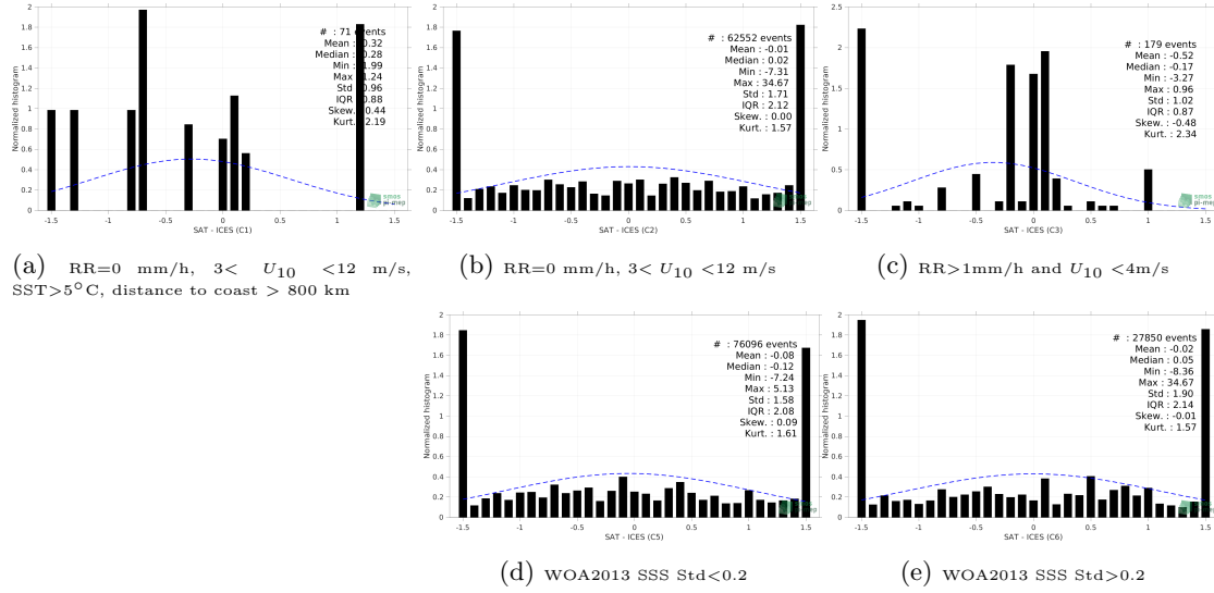
Figure 13: Normalized histogram of \Delta SSS (SMOS SSS L2 v700 (ESA) - ICES) for 5 different subdatasets corresponding to: RR=0 mm/h, 3 < U_{10} < 12 m/s, SST > 5°C, distance to coast > 800 km (a), RR=0 mm/h, 3 < U_{10} < 12 m/s (b), RR > 1mm/h and U_{10} < 4 m/s (c), WOA2013 SSS Std < 0.2 (d), WOA2013 SSS Std > 0.2 (e).
