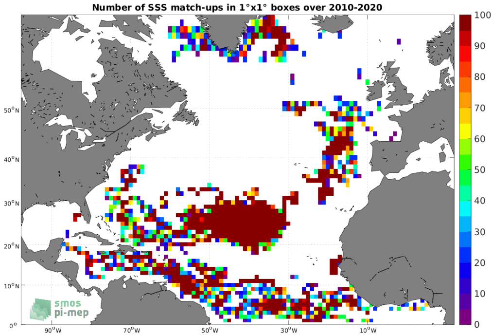
Figure 3: Number of SSS match-ups between Surface drifters SSS and the SMOS SSS L2 v700 (ESA) SSS product for the North Atlantic Ocean Pi-MEP region over 1^{\circ} \times 1^{\circ} boxes and for the full satellite product period.
