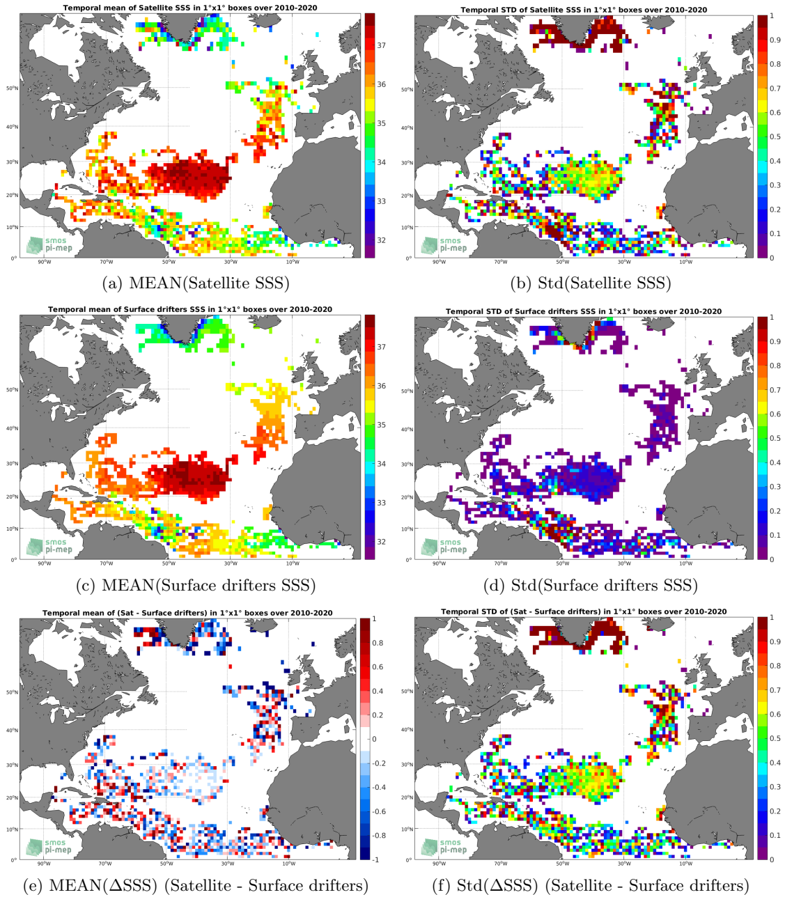
Figure 5: Temporal mean (left) and Std (right) of SSS from SMOS SSS L2 v700 (ESA) (top), Surface drifters (middle), and of \Delta SSS (Satellite - Surface drifters). Only match-up pairs are used to generate these maps.
