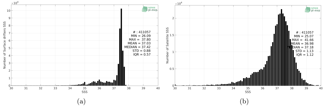
Figure 2: Histograms of SSS from Surface drifters (a) and SMOS SSS L2 v700 (ESA) (b) considering all match-up pairs per bins of 0.1 over the North Atlantic Ocean Pi-MEP region and for the full satellite product period.
