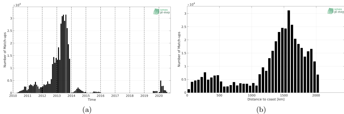
Figure 1: Number of match-ups between Surface drifters and SMOS SSS L2 v700 (ESA) SSS as a function of time (a) and as function of the distance to coast (b) over the North Atlantic Ocean Pi-MEP region and for the full satellite product period.
