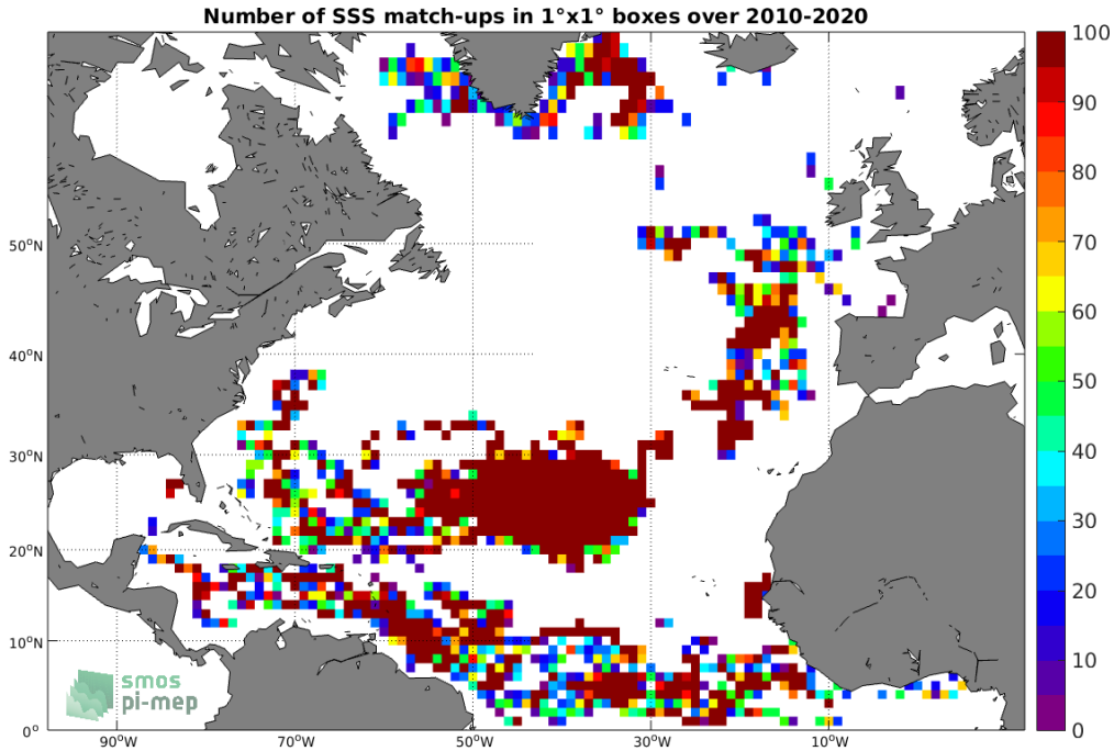
Figure 3: Number of SSS match-ups between Surface drifters SSS and the SMOS SSS L2 v700 (ESA) SSS product for the North Atlantic Ocean Pi-MEP region over 1^\circ \times 1^\circ boxes and for the full satellite product period.
