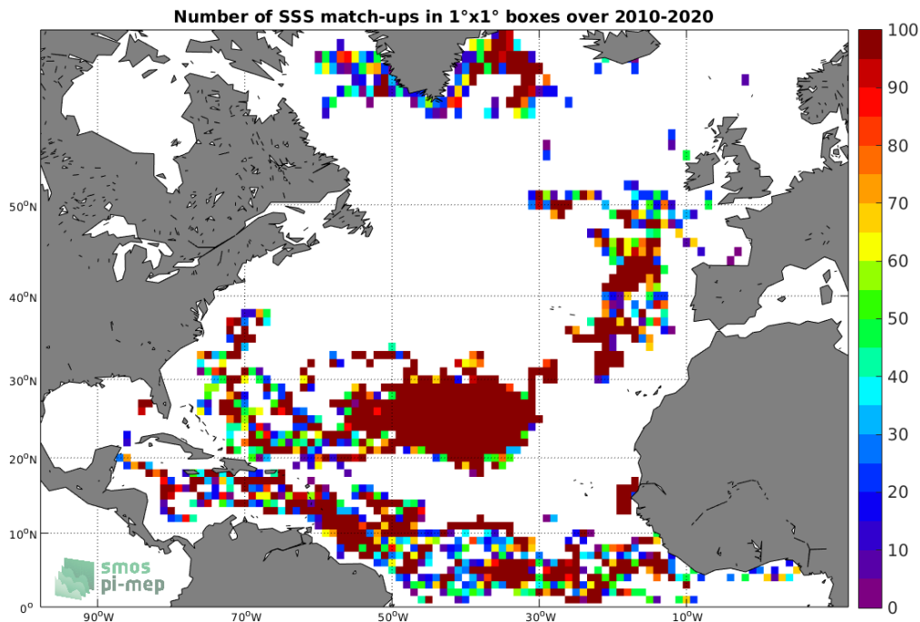
Figure 3: Number of SSS match-ups between Surface drifters SSS and the SMOS SSS L2 v700 (ESA) SSS product for the North Atlantic Ocean Pi-MEP region over 1°x1° boxes and for the full satellite product period.
