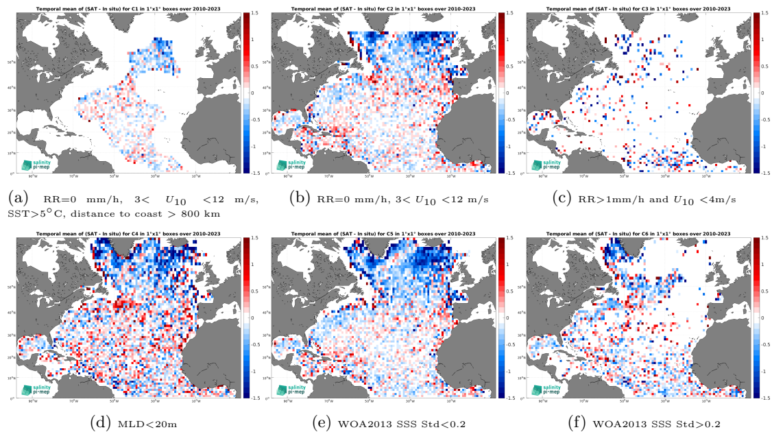
Figure 12: Temporal mean gridded over spatial boxes of size 1^\circ \times 1^\circ of \Delta\text{SSS} (SMOS SSS L2 v700 (ESA) - Argo) for 6 different subdatasets corresponding to:RR=0 mm/h, 3 < U_{10} < 12 m/s, SST > 5^\circ\text{C} , distance to coast > 800 km (a), RR=0 mm/h, 3 < U_{10} < 12 m/s (b), RR > 1 mm/h and U_{10} < 4 m/s (c),MLD < 20 m (d),WOA2013 SSS Std < 0.2 (e),WOA2013 SSS Std > 0.2 (f).
