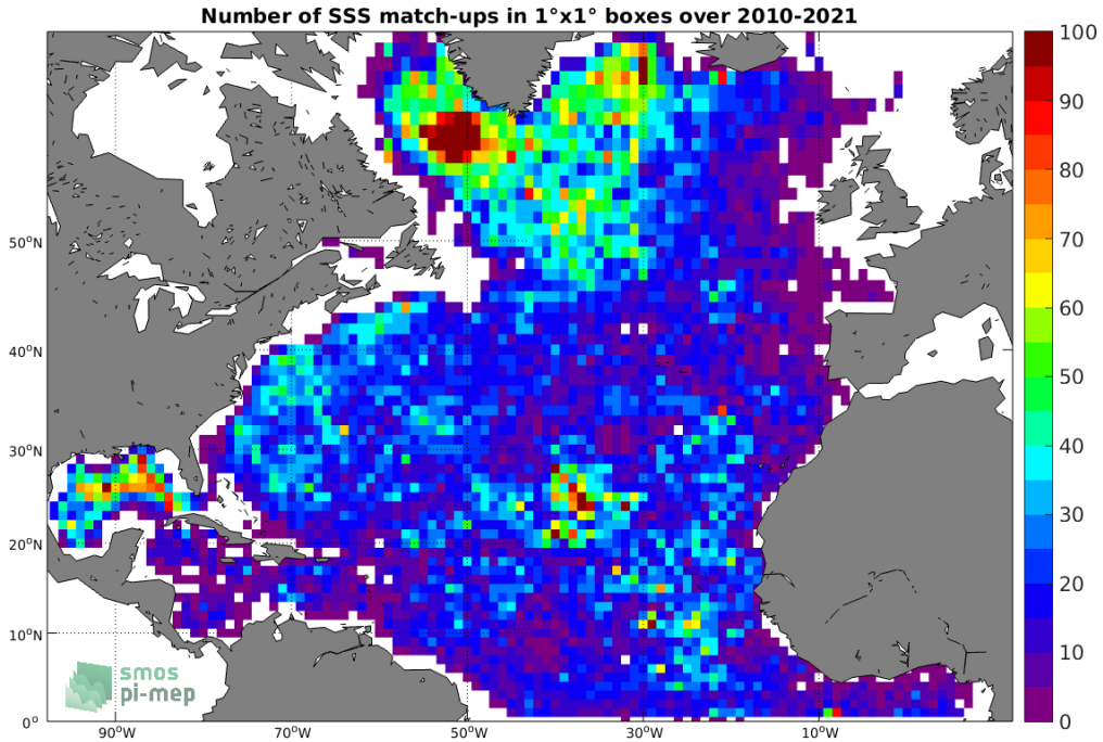
Figure 4: Number of SSS match-ups between Argo SSS and the SMOS SSS L2 v700 (ESA) SSS product for the North Atlantic Ocean Pi-MEP region over 1^\circ \times 1^\circ boxes and for the full satellite product period.
