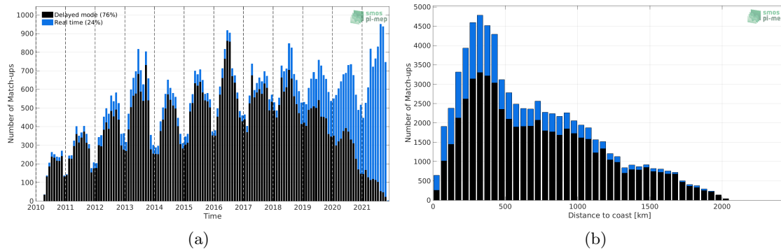
Figure 1: Number of match-ups between Argo and SMOS SSS L2 v700 (ESA) SSS as a function of time (a) and as function of the distance to coast (b) over the North Atlantic Ocean Pi-MEP region and for the full satellite product period.
