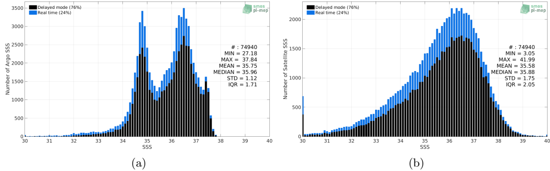
Figure 2: Histograms of SSS from Argo (a) and SMOS SSS L2 v700 (ESA) (b) considering all match-up pairs per bins of 0.1 over the North Atlantic Ocean Pi-MEP region and for the full satellite product period.
