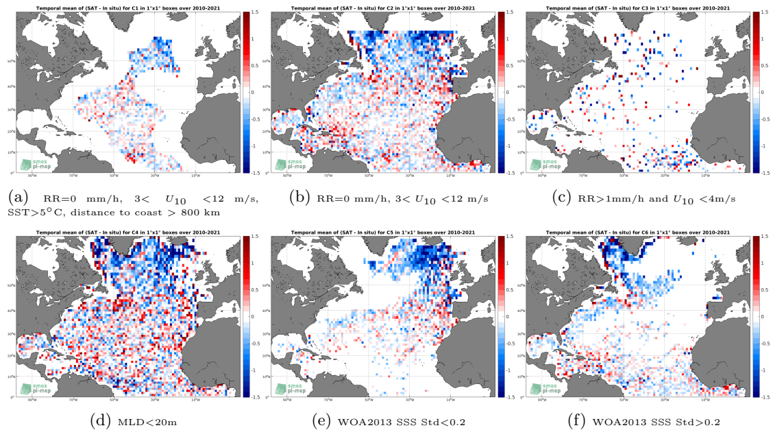
Figure 12: Temporal mean gridded over spatial boxes of size 1°x1° of \Delta SSS (SMOS SSS L2 v700 (ESA) - Argo) for 6 different subdatasets corresponding to:RR=0 mm/h, 3 < U_{10} < 12 m/s, SST>5°C, distance to coast > 800 km (a), RR=0 mm/h, 3 < U_{10} < 12 m/s (b), RR>1mm/h and U_{10} < 4 m/s (c),MLD<20m (d),WOA2013 SSS Std<0.2 (e),WOA2013 SSS Std>0.2 (f).
