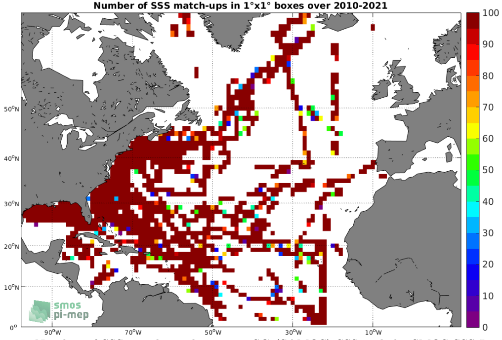
Figure 4: Number of SSS match-ups between TSG (SAMOS) SSS and the SMOS SSS L2 v662 (ESA) SSS product for the North Atlantic Ocean Pi-MEP region over 1^\circ \times 1^\circ boxes and for the full satellite product period.
