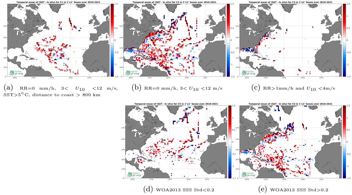
Figure 12: Temporal mean gridded over spatial boxes of size 1^\circ \times 1^\circ of \Delta SSS (SMOS SSS L2 v662 (ESA) - TSG (SAMOS)) for 5 different subdatasets corresponding to: RR=0 mm/h, 3 < U_{10} < 12 m/s, SST > 5^\circ\text{C} , distance to coast > 800 km (a), RR=0 mm/h, 3 < U_{10} < 12 m/s (b), RR > 1 mm/h and U_{10} < 4 m/s (c), WOA2013 SSS Std < 0.2 (d), WOA2013 SSS Std > 0.2 (e).
