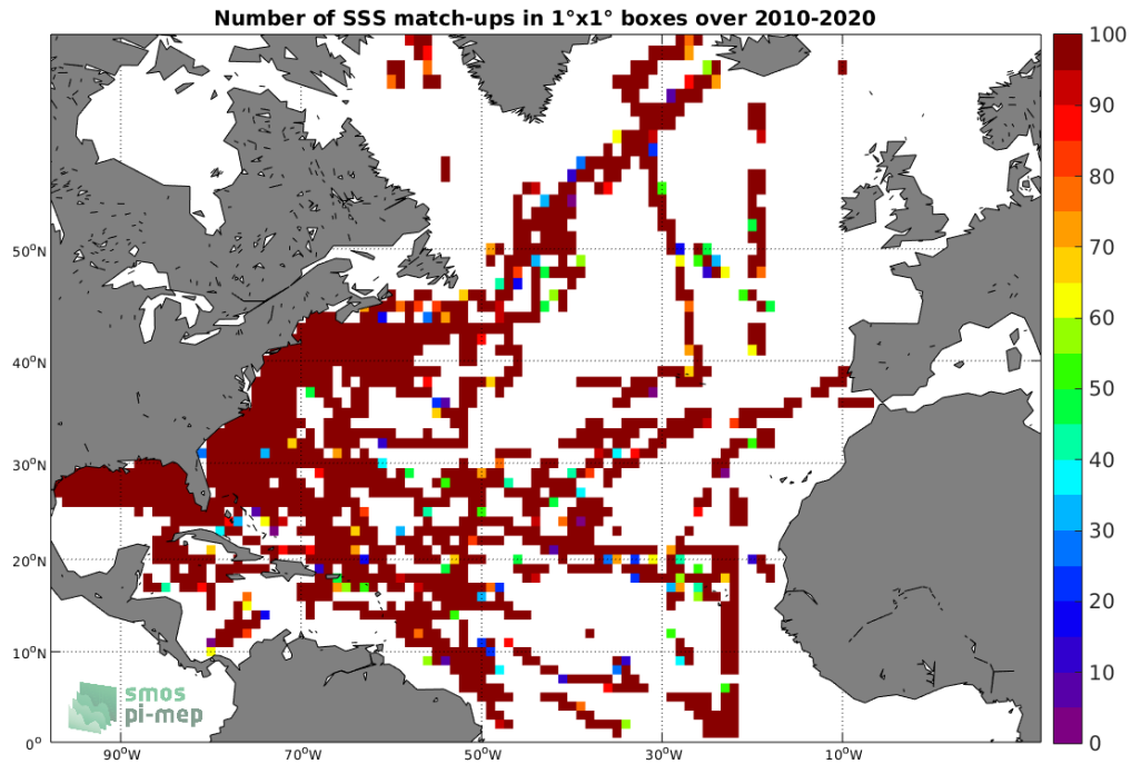
Figure 4: Number of SSS match-ups between TSG (SAMOS) SSS and the SMOS SSS L2 v662 (ESA) SSS product for the North Atlantic Ocean Pi-MEP region over 1°x1° boxes and for the full satellite product period.
