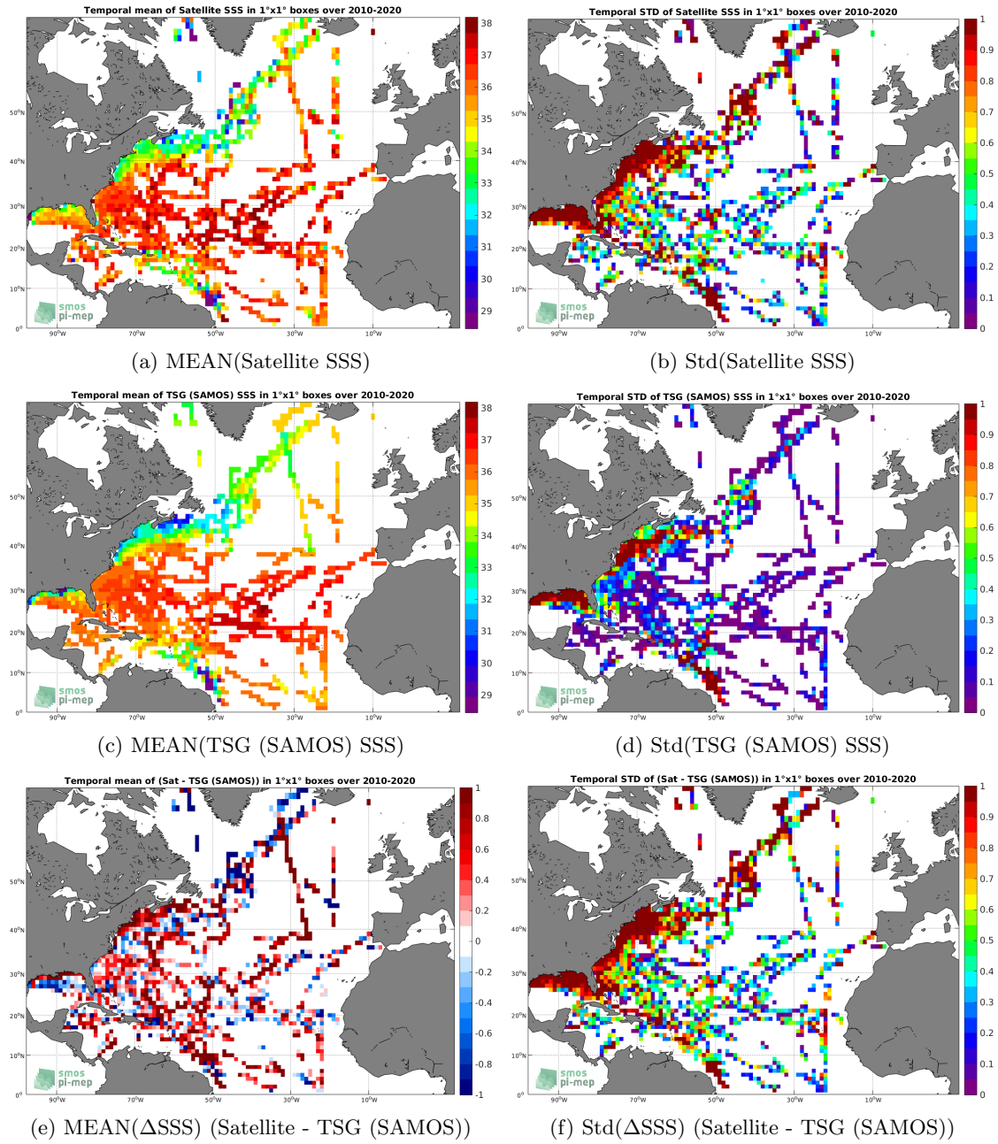
Figure 6: Temporal mean (left) and Std (right) of SSS from SMOS SSS L2 v662 (ESA) (top), TSG (SAMOS) (middle), and of \Delta SSS (Satellite - TSG (SAMOS)). Only match-up pairs are used to generate these maps.
