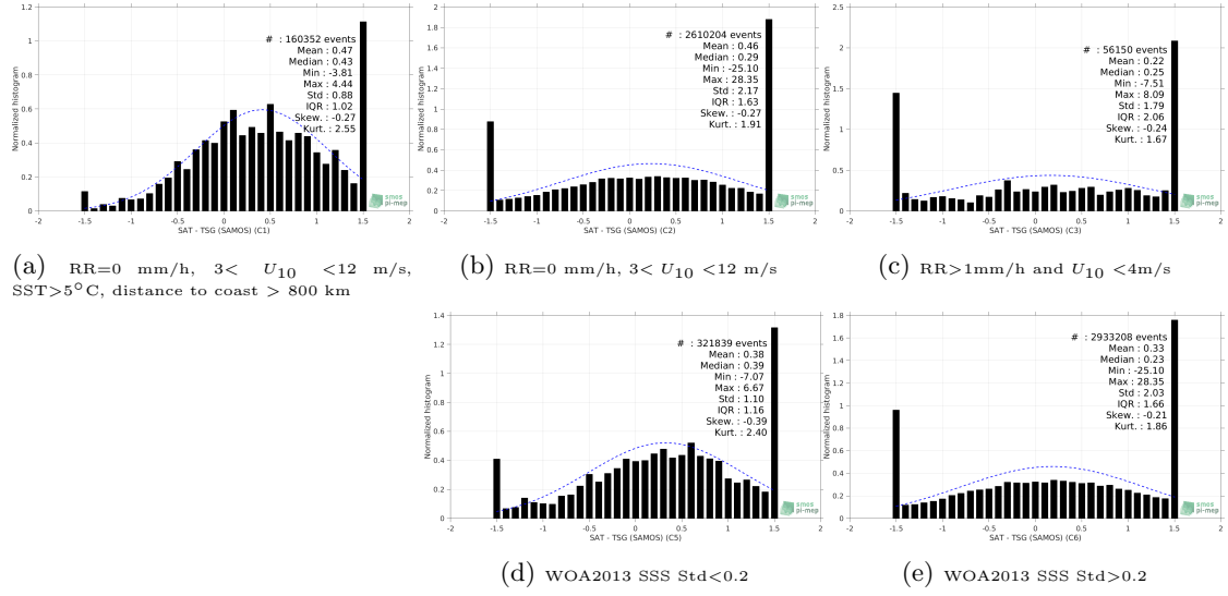
Figure 13: Normalized histogram of \Delta\text{SSS} (SMOS SSS L2 v662 (ESA) - TSG (SAMOS)) for 5 different subdatasets corresponding to: RR=0 mm/h, 3 < U_{10} < 12 m/s, SST>5°C, distance to coast > 800 km (a), RR=0 mm/h, 3 < U_{10} < 12 m/s (b), RR>1mm/h and U_{10} < 4 m/s (c), WOA2013 SSS Std<0.2 (d), WOA2013 SSS Std>0.2 (e).
