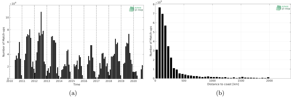
Figure 1: Number of match-ups between TSG (SAMOS) and SMOS SSS L2 v662 (ESA) SSS as a function of time (a) and as function of the distance to coast (b) over the North Atlantic Ocean Pi-MEP region and for the full satellite product period.
