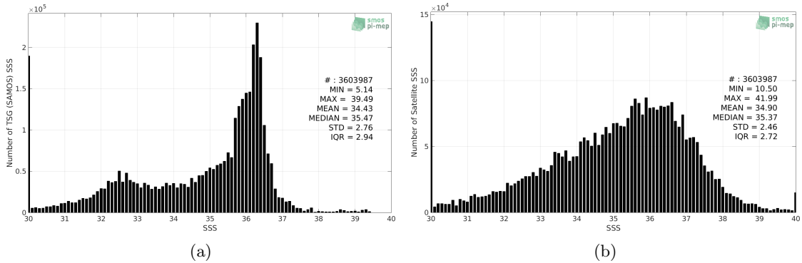
Figure 2: Histograms of SSS from TSG (SAMOS) (a) and SMOS SSS L2 v662 (ESA) (b) considering all match-up pairs per bins of 0.1 over the North Atlantic Ocean Pi-MEP region and for the full satellite product period.
