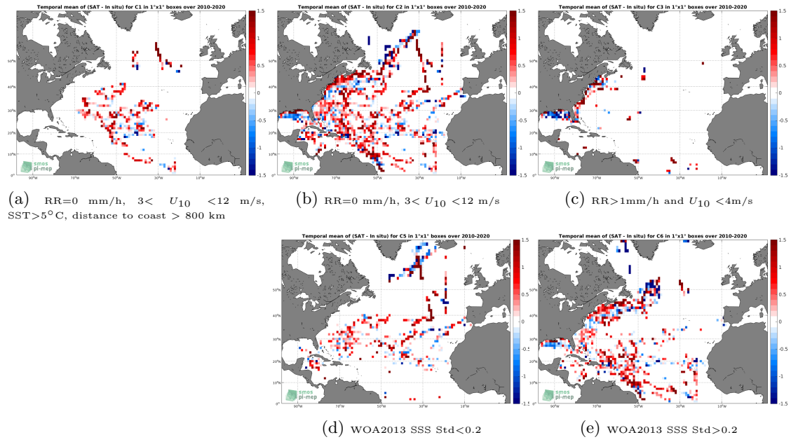
Figure 12: Temporal mean gridded over spatial boxes of size 1^\circ \times 1^\circ of \Delta SSS (SMOS SSS L2 v662 (ESA) - TSG (SAMOS)) for 5 different subdatasets corresponding to:RR=0 mm/h, 3 < U_{10} < 12 m/s, SST>5°C, distance to coast > 800 km (a), RR=0 mm/h, 3 < U_{10} < 12 m/s (b), RR>1mm/h and U_{10} < 4 m/s (c), WOA2013 SSS Std<0.2 (d), WOA2013 SSS Std>0.2 (e).
