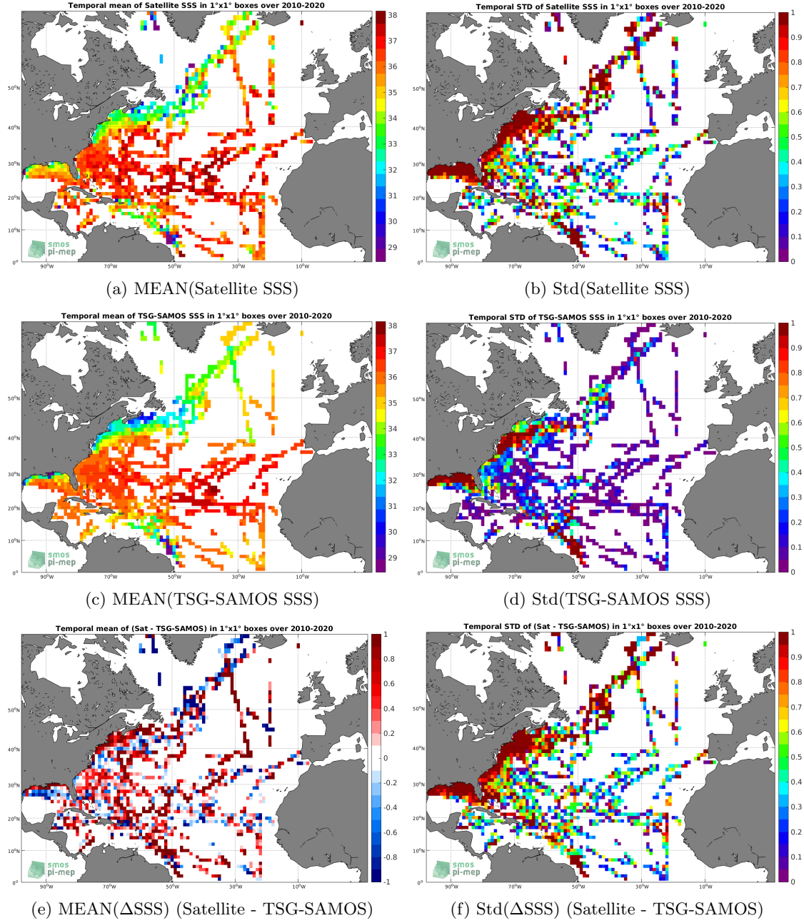
Figure 6: Temporal mean (left) and Std (right) of SSS from SMOS L2 v662 (ESA) (top), TSG-SAMOS (middle), and of \Delta SSS (Satellite - TSG-SAMOS). Only match-up pairs are used to generate these maps.
