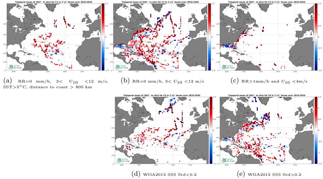
Figure 12: Temporal mean gridded over spatial boxes of size 1^\circ \times 1^\circ of \Delta SSS (SMOS L2 v662 (ESA) - TSG-SAMOS) for 5 different subdatasets corresponding to: RR=0 mm/h, 3 < U_{10} < 12 m/s, SST > 5^\circ C , distance to coast > 800 km (a), RR=0 mm/h, 3 < U_{10} < 12 m/s (b), RR > 1 mm/h and U_{10} < 4 m/s (c), WOA2013 SSS Std < 0.2 (d), WOA2013 SSS Std > 0.2 (e).
