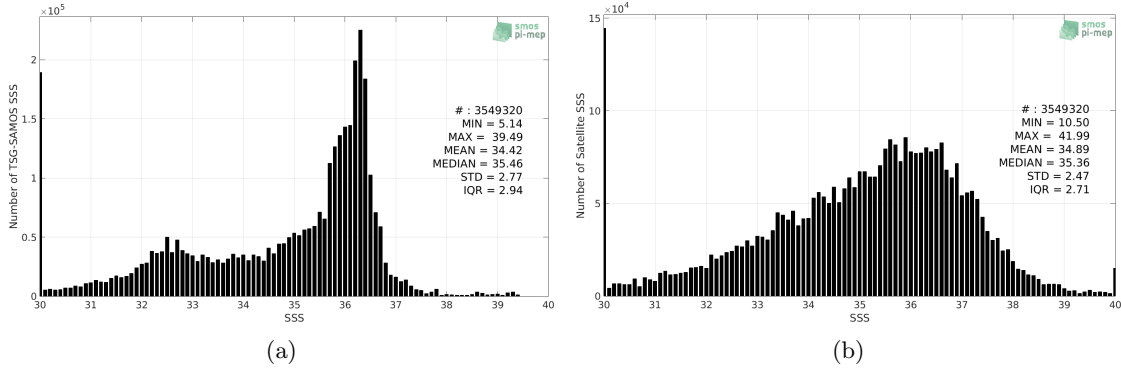
Figure 2: Histograms of SSS from TSG-SAMOS (a) and SMOS L2 v662 (ESA) (b) considering all match-up pairs per bins of 0.1 over the North Atlantic Ocean Pi-MEP region and for the full satellite product period.
