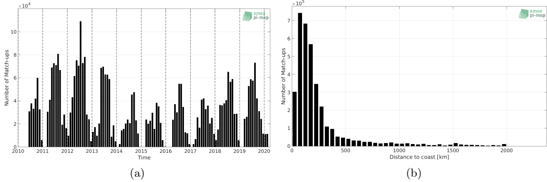
Figure 1: Number of match-ups between TSG-SAMOS and SMOS L2 v662 (ESA) SSS as a function of time (a) and as function of the distance to coast (b) over the North Atlantic Ocean Pi-MEP region and for the full satellite product period.
