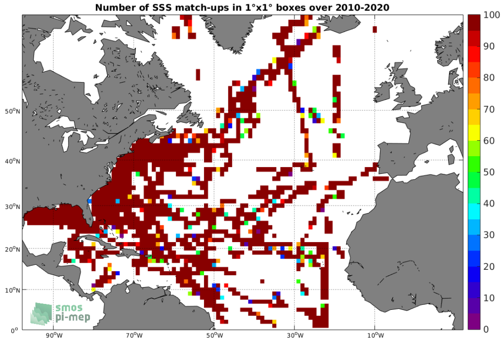
Figure 4: Number of SSS match-ups between TSG-SAMOS SSS and the SMOS L2 v662 (ESA) SSS product for the North Atlantic Ocean Pi-MEP region over 1°x1° boxes and for the full satellite product period.
