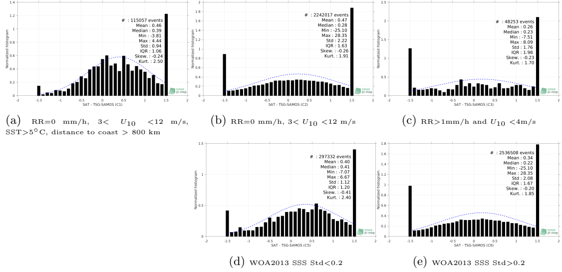
Figure 13: Normalized histogram of \Delta\text{SSS} (SMOS-L2-DPGS-v662 - TSG-SAMOS) for 5 different subdatasets corresponding to: RR=0 mm/h, 3 < U_{10} < 12 m/s, SST > 5^\circ\text{C} , distance to coast > 800 km (a), RR=0 mm/h, 3 < U_{10} < 12 m/s (b), RR > 1\text{mm/h} and U_{10} < 4\text{m/s} (c), WOA2013 SSS \text{Std} < 0.2 (d), WOA2013 SSS \text{Std} > 0.2 (e).
