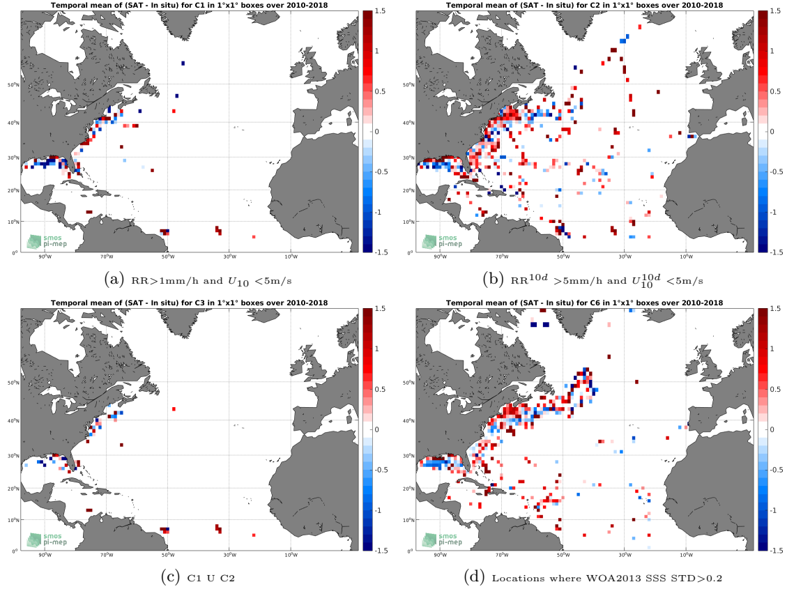
Figure 12: Temporal mean gridded over spatial boxes of size 1^\circ \times 1^\circ of \Delta SSS (SMOS-L2-DPGS-v662 - TSG-SAMOS) for 4 different subdatasets corresponding to: RR > 1\text{mm/h} and U_{10} < 5\text{m/s} (a), RR^{10d} > 5\text{mm/h} and U_{10}^{10d} < 5\text{m/s} (b), C1 U C2 (c), Locations where WOA2013 SSS STD > 0.2 (d).
