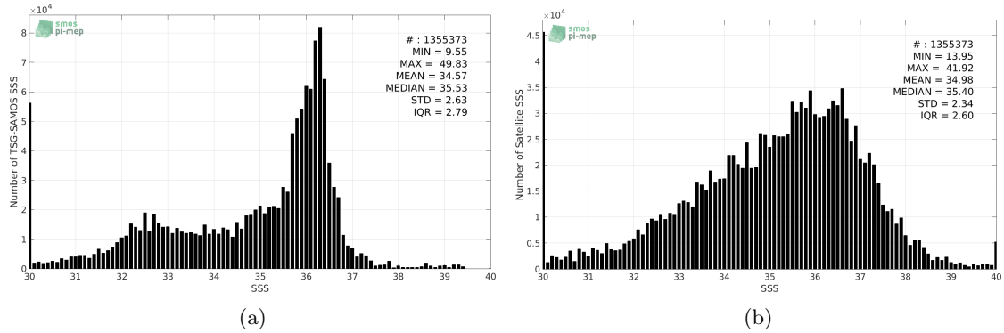
Figure 2: Histograms of SSS from TSG-SAMOS (a) and SMOS-L2-DPGS-v662 (b) considering all match-up pairs per bins of 0.1 over the North Atlantic Ocean Pi-MEP region and for the full satellite product period.
