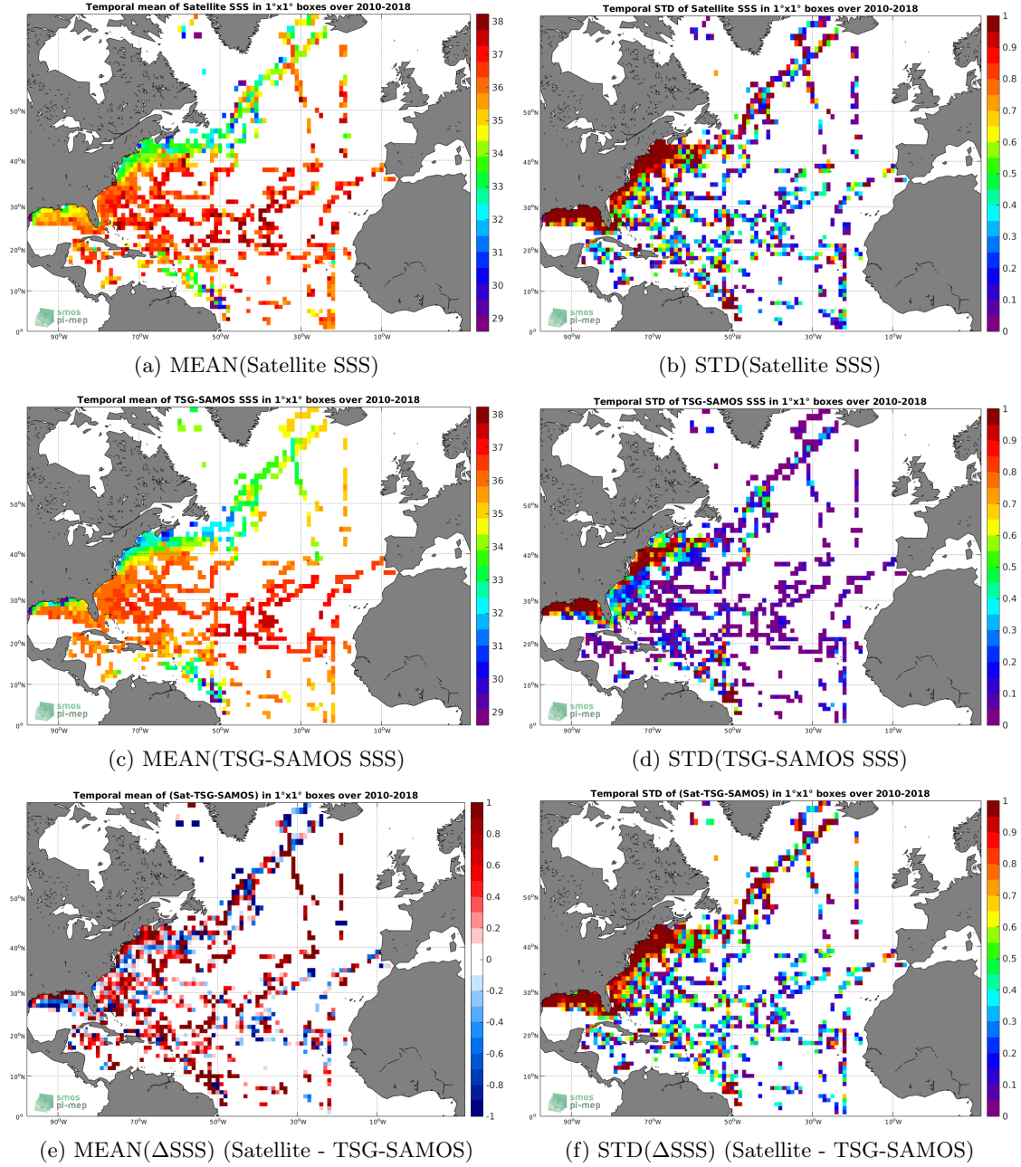
Figure 6: Temporal mean (left) and STD (right) of SSS from SMOS-L2-DPGS-v662 (top), TSG-SAMOS (middle), and of \Delta SSS (Satellite - TSG-SAMOS). Only match-up pairs are used to generate these maps.
