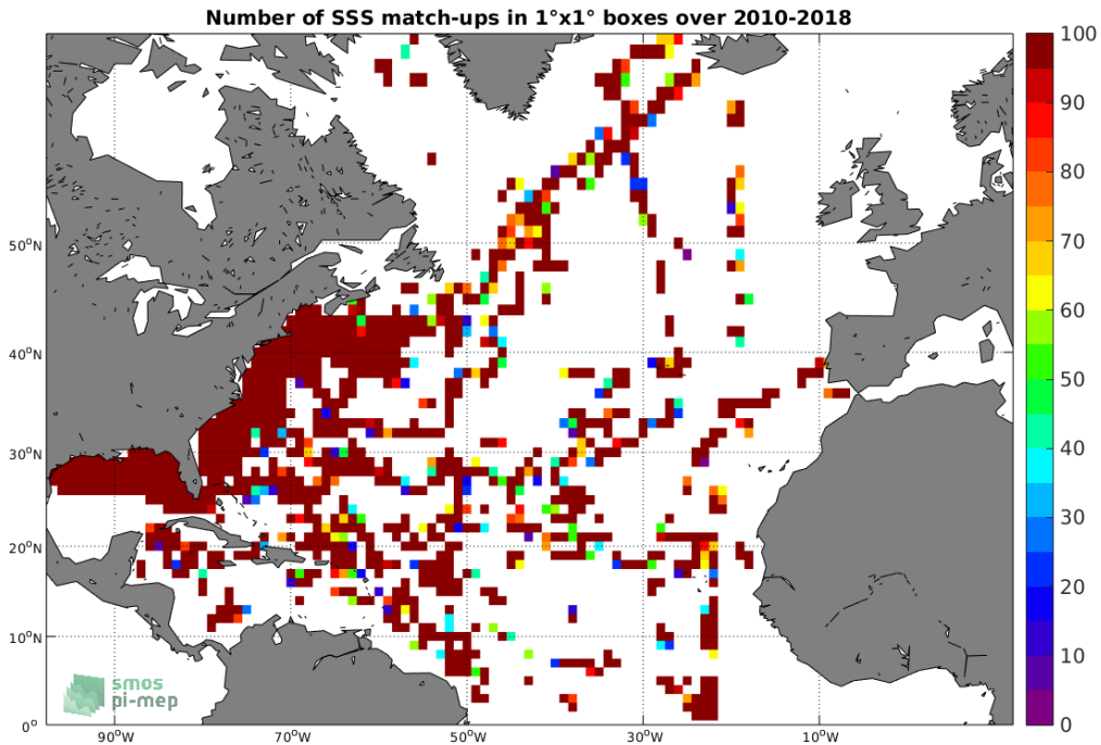
Figure 4: Number of SSS match-ups between TSG-SAMOS SSS and the SMOS-L2-DPGS-v662 SSS product for the North Atlantic Ocean Pi-MEP region over 1^\circ \times 1^\circ boxes and for the full satellite product period.
