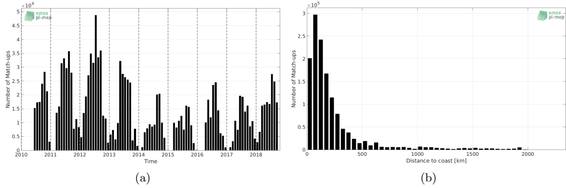
Figure 1: Number of match-ups between TSG-SAMOS and SMOS-L2-DPGS-v662 SSS as a function of time (a) and as function of the distance to coast (b) over the North Atlantic Ocean Pi-MEP region and for the full satellite product period.
