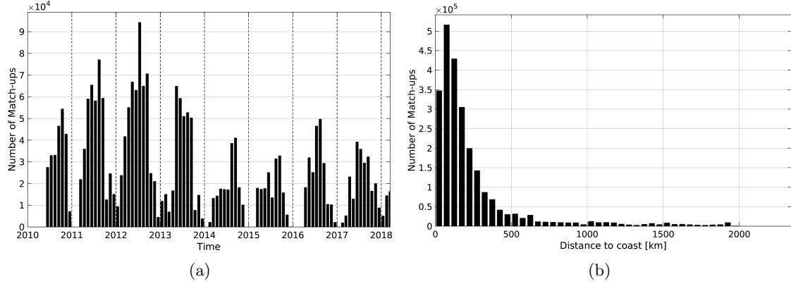
Figure 1: Number of match-ups between TSG-SAMOS and SMOS-L2-DPGS-v662 SSS as a function of time (a) and as function of the distance to coast (b) over the North Atlantic Ocean Pi-MEP region and for the full satellite product period.
