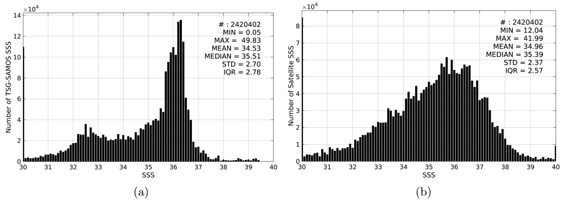
Figure 2: Histograms of SSS from TSG-SAMOS (a) and SMOS-L2-DPGS-v662 (b) considering all match-up pairs per bins of 0.1 over the North Atlantic Ocean Pi-MEP region and for the full satellite product period.
