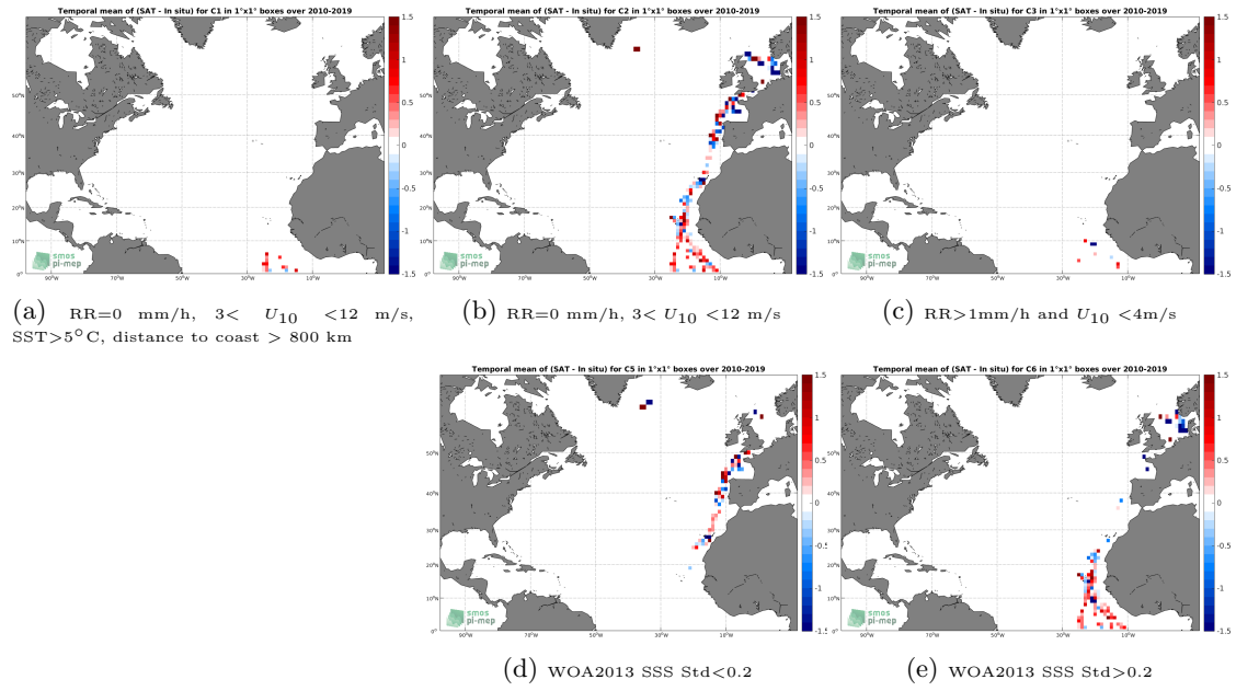
Figure 12: Temporal mean gridded over spatial boxes of size 1^\circ \times 1^\circ of \Delta SSS (SMOS SSS L2 v662 (ESA) - TSG (Polarstern)) for 5 different subdatasets corresponding to: RR=0 mm/h, 3 < U_{10} < 12 m/s, SST > 5^\circ\text{C} , distance to coast > 800 km (a), RR=0 mm/h, 3 < U_{10} < 12 m/s (b), RR > 1 mm/h and U_{10} < 4 m/s (c), WOA2013 SSS Std < 0.2 (d), WOA2013 SSS Std > 0.2 (e).
