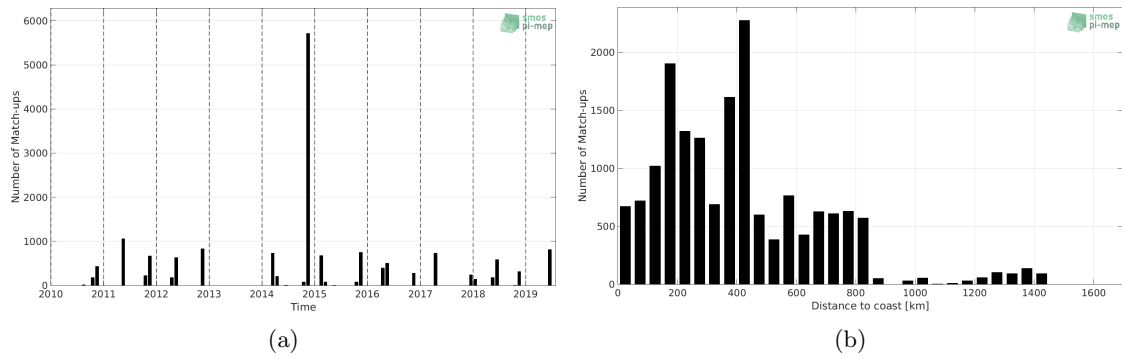
Figure 1: Number of match-ups between TSG (Polarstern) and SMOS SSS L2 v662 (ESA) SSS as a function of time (a) and as function of the distance to coast (b) over the North Atlantic Ocean Pi-MEP region and for the full satellite product period.
