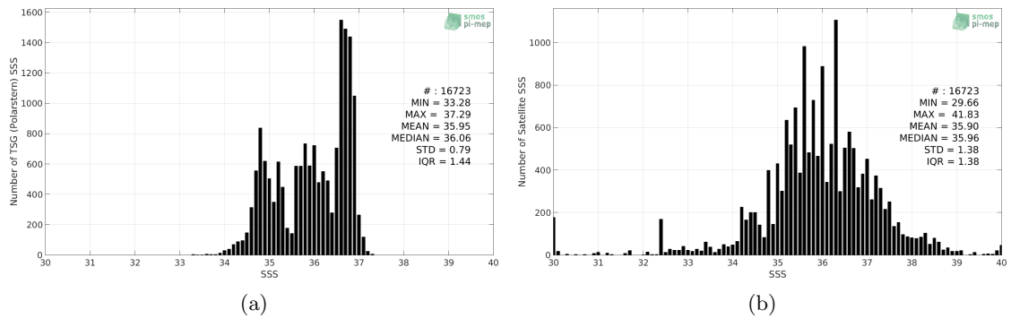
Figure 2: Histograms of SSS from TSG (Polarstern) (a) and SMOS SSS L2 v662 (ESA) (b) considering all match-up pairs per bins of 0.1 over the North Atlantic Ocean Pi-MEP region and for the full satellite product period.
