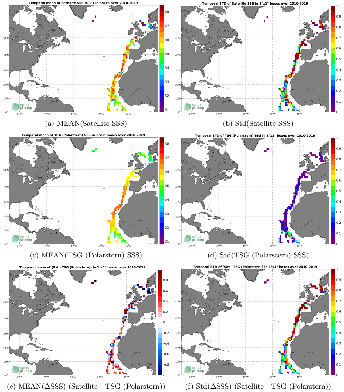
Figure 6: Temporal mean (left) and Std (right) of SSS from SMOS SSS L2 v662 (ESA) (top), TSG (Polarstern) (middle), and of \Delta SSS (Satellite - TSG (Polarstern)). Only match-up pairs are used to generate these maps.
