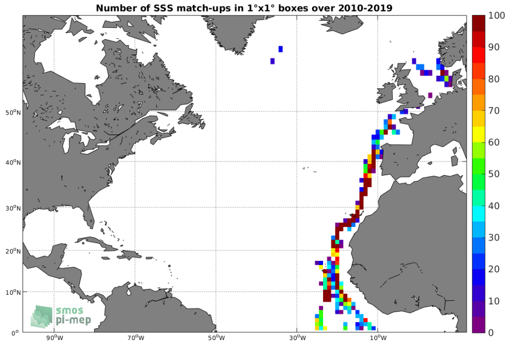
Figure 4: Number of SSS match-ups between TSG (Polarstern) SSS and the SMOS SSS L2 v662 (ESA) SSS product for the North Atlantic Ocean Pi-MEP region over 1°x1° boxes and for the full satellite product period.
