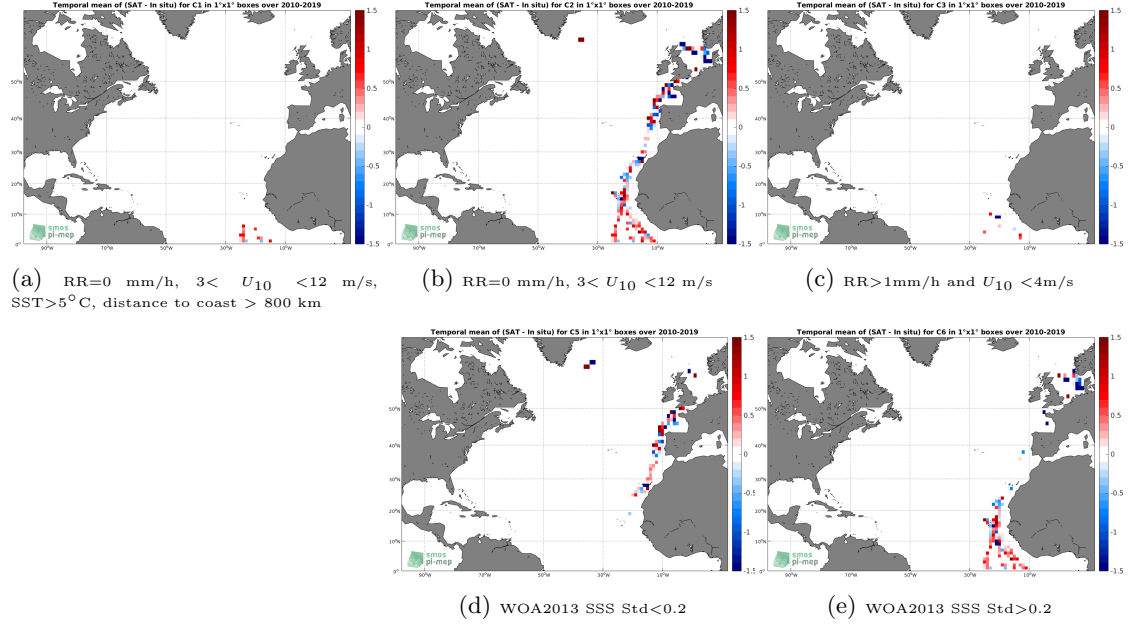
Figure 12: Temporal mean gridded over spatial boxes of size 1^\circ \times 1^\circ of \Delta SSS (SMOS L2 v662 (ESA) - TSG-POLARSTERN) for 5 different subdatasets corresponding to:RR=0 mm/h, 3 < U_{10} < 12 m/s, SST >5^\circ\text{C} , distance to coast > 800 km (a), RR=0 mm/h, 3 < U_{10} < 12 m/s (b), RR >1 mm/h and U_{10} < 4 m/s (c), WOA2013 SSS Std <0.2 (d), WOA2013 SSS Std >0.2 (e).
