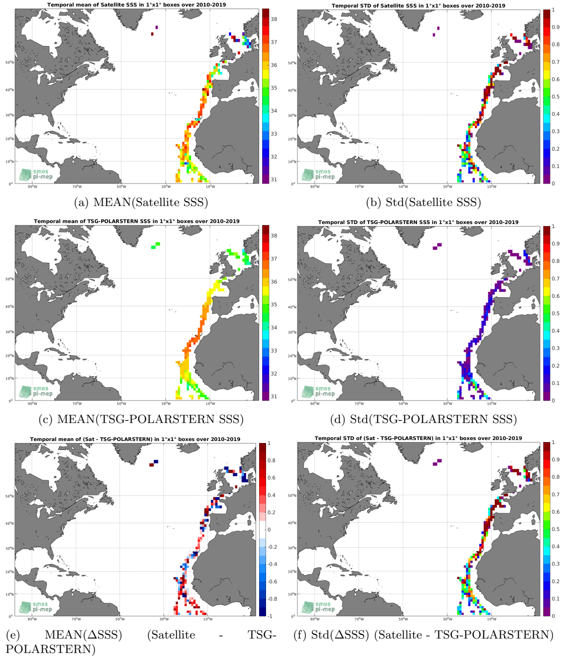
Figure 6: Temporal mean (left) and Std (right) of SSS from SMOS L2 v662 (ESA) (top), TSG-POLARSTERN (middle), and of \Delta SSS (Satellite - TSG-POLARSTERN). Only match-up pairs are used to generate these maps.
