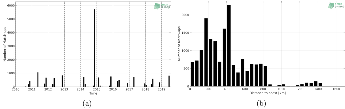
Figure 1: Number of match-ups between TSG-POLARSTERN and SMOS L2 v662 (ESA) SSS as a function of time (a) and as function of the distance to coast (b) over the North Atlantic Ocean Pi-MEP region and for the full satellite product period.
