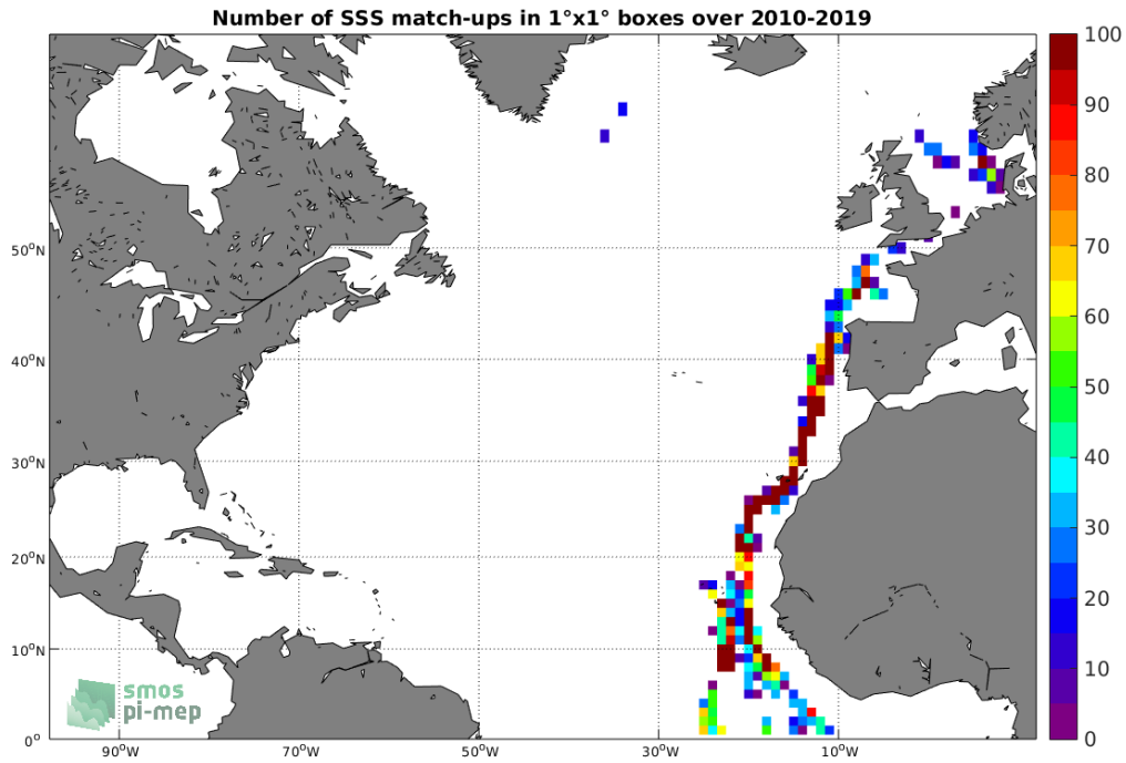
Figure 4: Number of SSS match-ups between TSG-POLARSTERN SSS and the SMOS L2 v662 (ESA) SSS product for the North Atlantic Ocean Pi-MEP region over 1^\circ \times 1^\circ boxes and for the full satellite product period.
