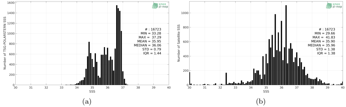
Figure 2: Histograms of SSS from TSG-POLARSTERN (a) and SMOS L2 v662 (ESA) (b) considering all match-up pairs per bins of 0.1 over the North Atlantic Ocean Pi-MEP region and for the full satellite product period.
