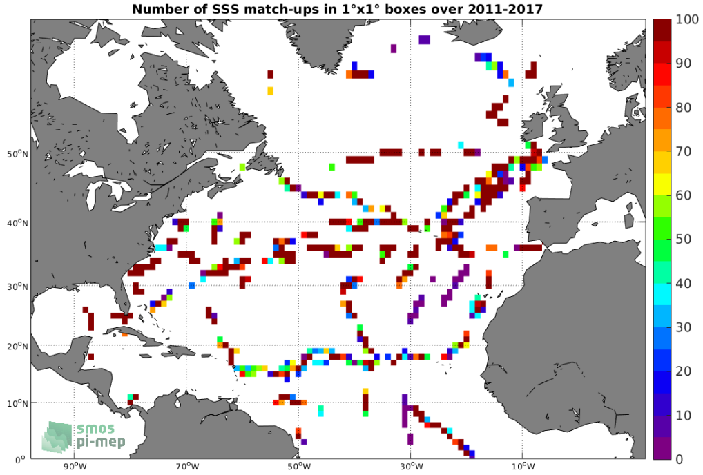
Figure 4: Number of SSS match-ups between TSG (GOSUD-Sailing-ship) SSS and the SMOS SSS L2 v662 (ESA) SSS product for the North Atlantic Ocean Pi-MEP region over 1^\circ \times 1^\circ boxes and for the full satellite product period.
