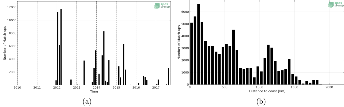
Figure 1: Number of match-ups between TSG (GOSUD-Sailing-ship) and SMOS SSS L2 v662 (ESA) SSS as a function of time (a) and as function of the distance to coast (b) over the North Atlantic Ocean Pi-MEP region and for the full satellite product period.
