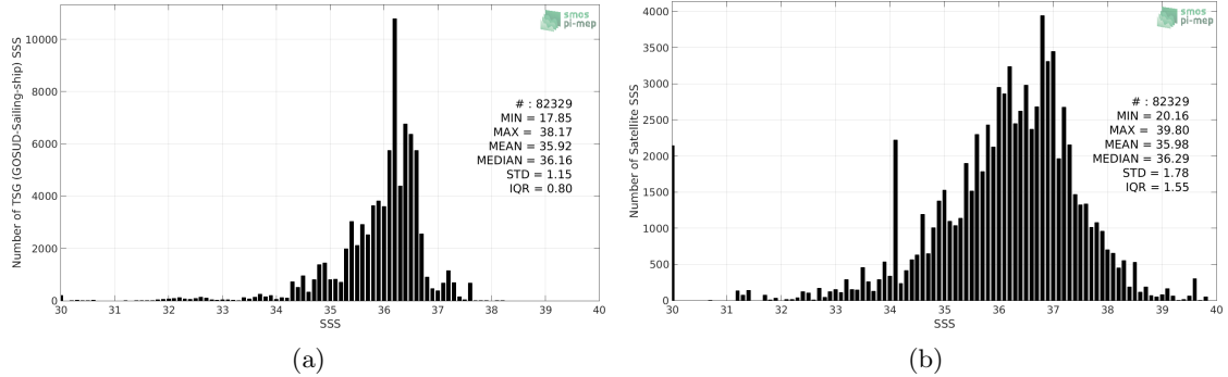
Figure 2: Histograms of SSS from TSG (GOSUD-Sailing-ship) (a) and SMOS SSS L2 v662 (ESA) (b) considering all match-up pairs per bins of 0.1 over the North Atlantic Ocean Pi-MEP region and for the full satellite product period.
