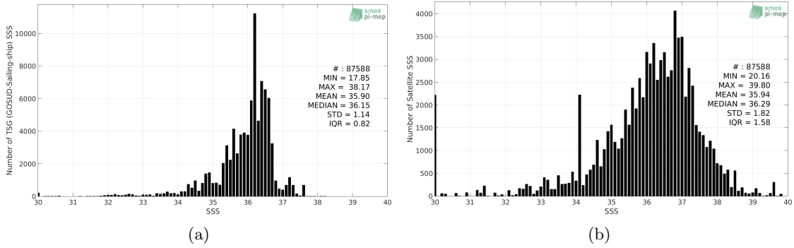
Figure 2: Histograms of SSS from TSG (GOSUD-Sailing-ship) (a) and SMOS SSS L2 v662 (ESA) (b) considering all match-up pairs per bins of 0.1 over the North Atlantic Ocean Pi-MEP region and for the full satellite product period.
