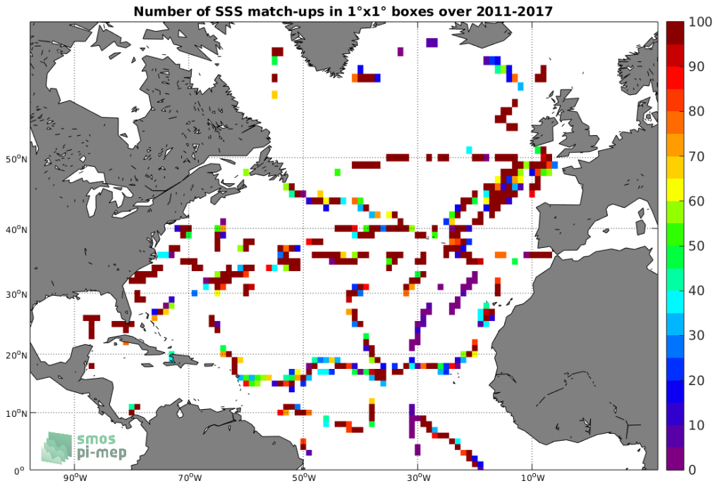
Figure 4: Number of SSS match-ups between TSG-GOSUD-Sailing-ship SSS and the SMOS L2 v662 (ESA) SSS product for the North Atlantic Ocean Pi-MEP region over 1°x1° boxes and for the full satellite product period.
