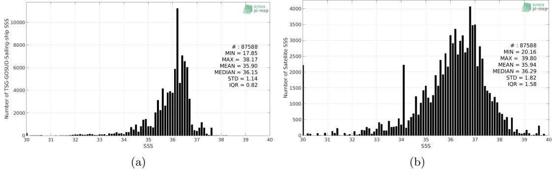
Figure 2: Histograms of SSS from TSG-GOSUD-Sailing-ship (a) and SMOS L2 v662 (ESA) (b) considering all match-up pairs per bins of 0.1 over the North Atlantic Ocean Pi-MEP region and for the full satellite product period.
