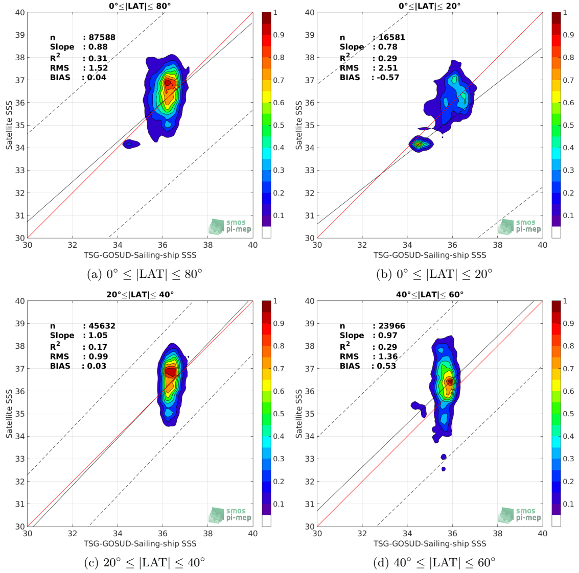
Figure 9: Contour maps of the concentration of SMOS L2 v662 (ESA) SSS (y-axis) versus TSG-GOSUD-Sailing-ship SSS (x-axis) at match-up pairs for different latitude bands. For each plot, the red line shows x=y . The black thin and dashed lines indicate a linear fit through the data cloud and the \pm 95\% confidence levels, respectively. The number match-up pairs n , the slope and R^2 coefficient of the linear fit, the root mean square (RMS) and the mean bias between satellite and in situ data are indicated for each latitude band in each plots.
