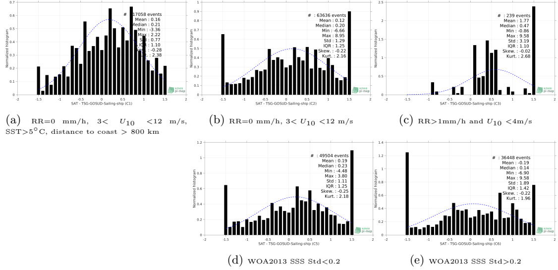
Figure 13: Normalized histogram of \Delta SSS (SMOS L2 v662 (ESA) - TSG-GOSUD-Sailing-ship) for 5 different subdatasets corresponding to: RR=0 mm/h, 3 < U_{10} < 12 m/s, SST>5°C, distance to coast > 800 km (a), RR=0 mm/h, 3 < U_{10} < 12 m/s (b), RR>1mm/h and U_{10} < 4 m/s (c), WOA2013 SSS Std<0.2 (d), WOA2013 SSS Std>0.2 (e).
