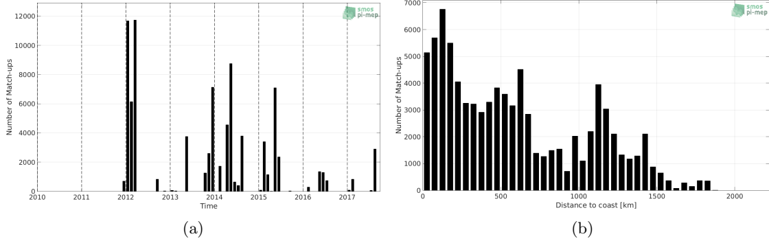
Figure 1: Number of match-ups between TSG-GOSUD-Sailing-ship and SMOS L2 v662 (ESA) SSS as a function of time (a) and as function of the distance to coast (b) over the North Atlantic Ocean Pi-MEP region and for the full satellite product period.
