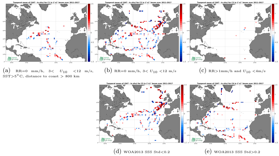
Figure 12: Temporal mean gridded over spatial boxes of size 1^\circ \times 1^\circ of \Delta SSS (SMOS L2 v662 (ESA) - TSG-GOSUD-Sailing-ship) for 5 different subdatasets corresponding to: RR=0 mm/h, 3 < U_{10} < 12 m/s, SST > 5^\circ\text{C} , distance to coast > 800 km (a), RR=0 mm/h, 3 < U_{10} < 12 m/s (b), RR > 1 mm/h and U_{10} < 4 m/s (c), WOA2013 SSS Std < 0.2 (d), WOA2013 SSS Std > 0.2 (e).
