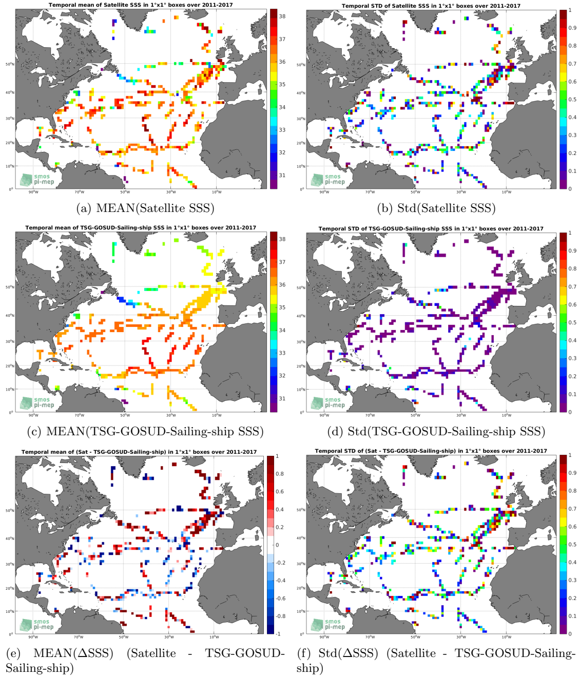
Figure 6: Temporal mean (left) and Std (right) of SSS from SMOS L2 v662 (ESA) (top), TSG-GOSUD-Sailing-ship (middle), and of \Delta SSS (Satellite - TSG-GOSUD-Sailing-ship). Only match-up pairs are used to generate these maps.
