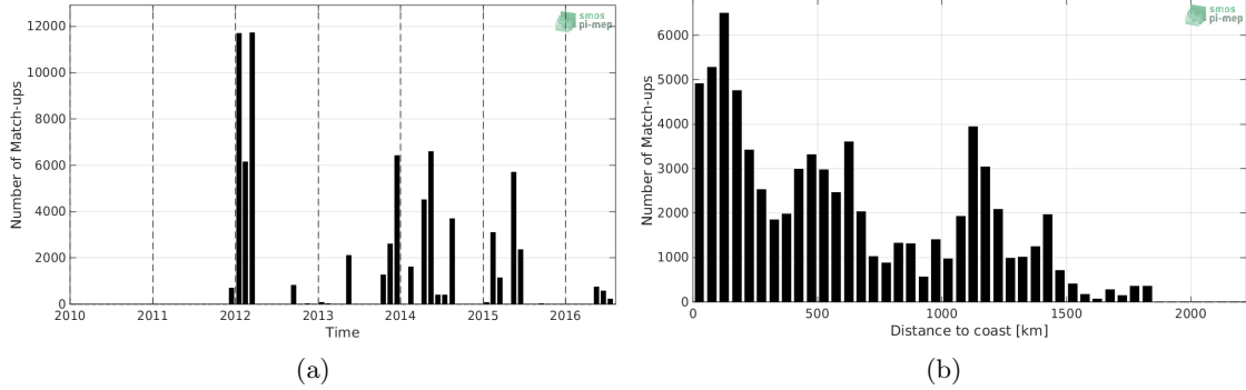
Figure 1: Number of match-ups between TSG-GOSUD-Sailing-ship and SMOS-L2-DPGS-v662 SSS as a function of time (a) and as function of the distance to coast (b) over the North Atlantic Ocean Pi-MEP region and for the full satellite product period.
