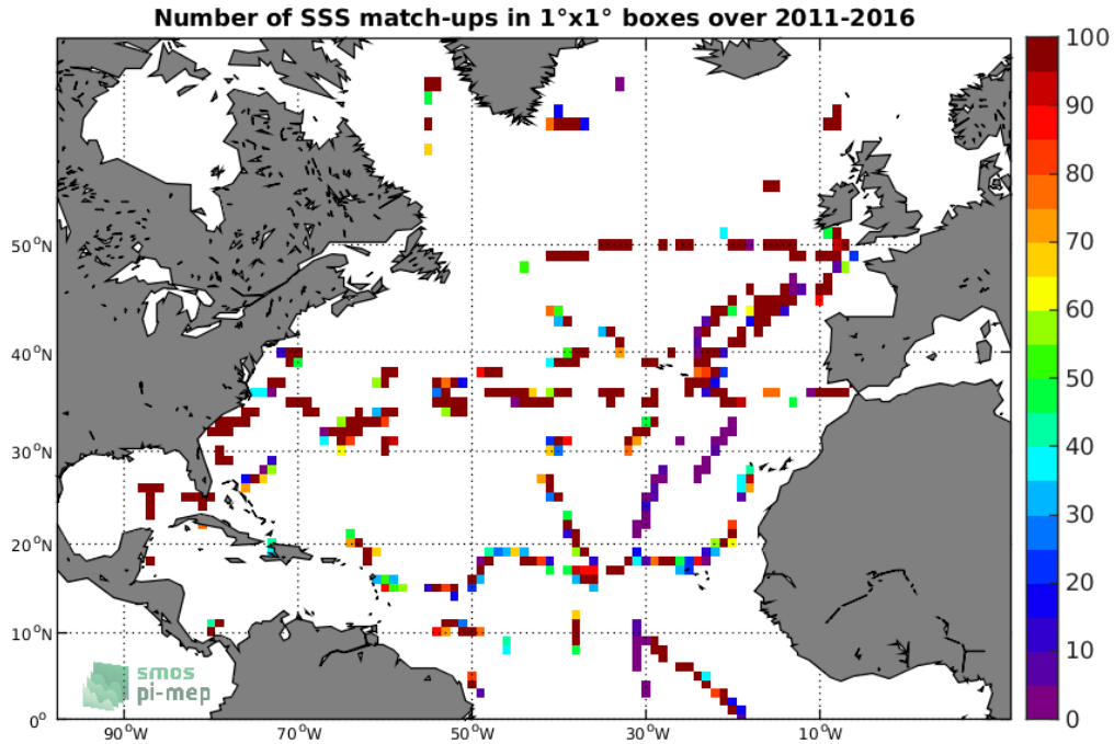
Figure 4: Number of SSS match-ups between TSG-GOSUD-Sailing-ship SSS and the SMOS-L2-DPGS-v662 SSS product for the North Atlantic Ocean Pi-MEP region over 1°x1° boxes and for the full satellite product period.
