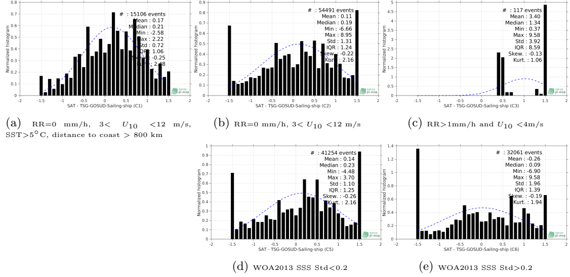
Figure 13: Normalized histogram of \Delta\text{SSS} (SMOS-L2-DPGS-v662 - TSG-GOSUD-Sailing-ship) for 5 different subdatasets corresponding to: RR=0 mm/h, 3 < U_{10} < 12 m/s, SST > 5^{\circ}\text{C} , distance to coast > 800 km (a), RR=0 mm/h, 3 < U_{10} < 12 m/s (b), RR > 1\text{mm/h} and U_{10} < 4\text{m/s} (c), WOA2013 SSS \text{Std} < 0.2 (d), WOA2013 SSS \text{Std} > 0.2 (e).
