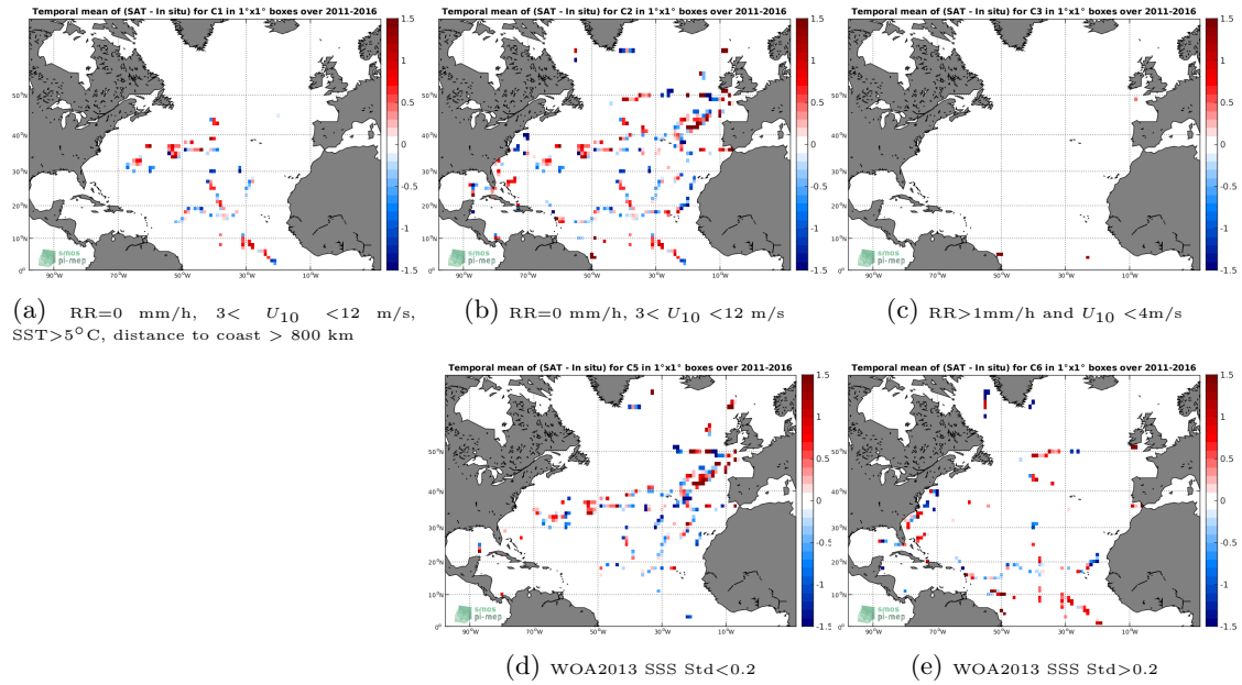
Figure 12: Temporal mean gridded over spatial boxes of size 1^\circ \times 1^\circ of \Delta SSS (SMOS-L2-DPGS-v662 - TSG-GOSUD-Sailing-ship) for 5 different subdatasets corresponding to:RR=0 mm/h, 3 < U_{10} < 12 m/s, SST >5^\circ\text{C} , distance to coast > 800 km (a), RR=0 mm/h, 3 < U_{10} < 12 m/s (b), RR >1 mm/h and U_{10} < 4 m/s (c), WOA2013 SSS Std <0.2 (d), WOA2013 SSS Std >0.2 (e).
