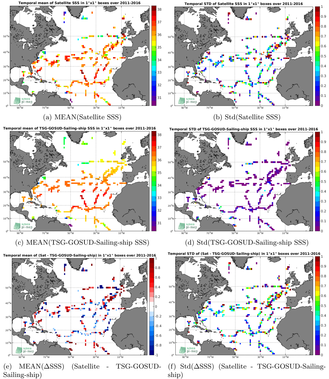
Figure 6: Temporal mean (left) and Std (right) of SSS from SMOS-L2-DPGS-v662 (top), TSG-GOSUD-Sailing-ship (middle), and of \Delta SSS (Satellite - TSG-GOSUD-Sailing-ship). Only match-up pairs are used to generate these maps.
