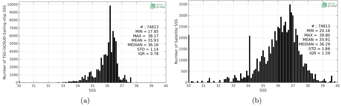
Figure 2: Histograms of SSS from TSG-GOSUD-Sailing-ship (a) and SMOS-L2-DPGS-v662 (b) considering all match-up pairs per bins of 0.1 over the North Atlantic Ocean Pi-MEP region and for the full satellite product period.
