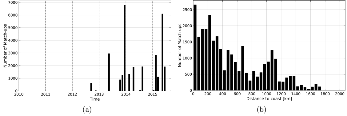
Figure 1: Number of match-ups between TSG-GOSUD-Sailing-ship and SMOS-L2-DPGS-v662 SSS as a function of time (a) and as function of the distance to coast (b) over the North Atlantic Ocean Pi-MEP region and for the full satellite product period.
