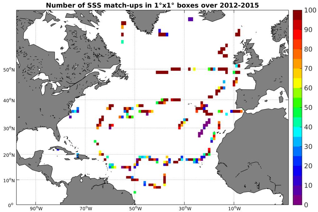
Figure 4: Number of SSS match-ups between TSG-GOSUD-Sailing-ship SSS and the SMOS-L2-DPGS-v662 SSS product for the North Atlantic Ocean Pi-MEP region over 1^\circ \times 1^\circ boxes and for the full satellite product period.
