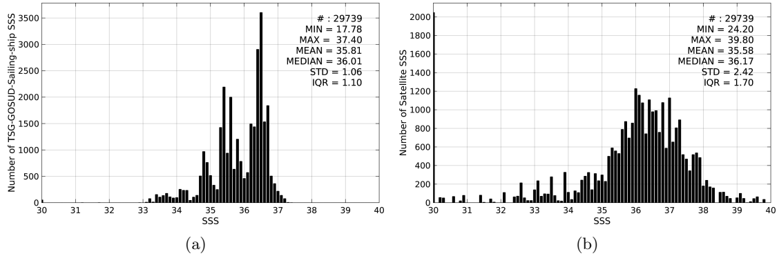
Figure 2: Histograms of SSS from TSG-GOSUD-Sailing-ship (a) and SMOS-L2-DPGS-v662 (b) considering all match-up pairs per bins of 0.1 over the North Atlantic Ocean Pi-MEP region and for the full satellite product period.
