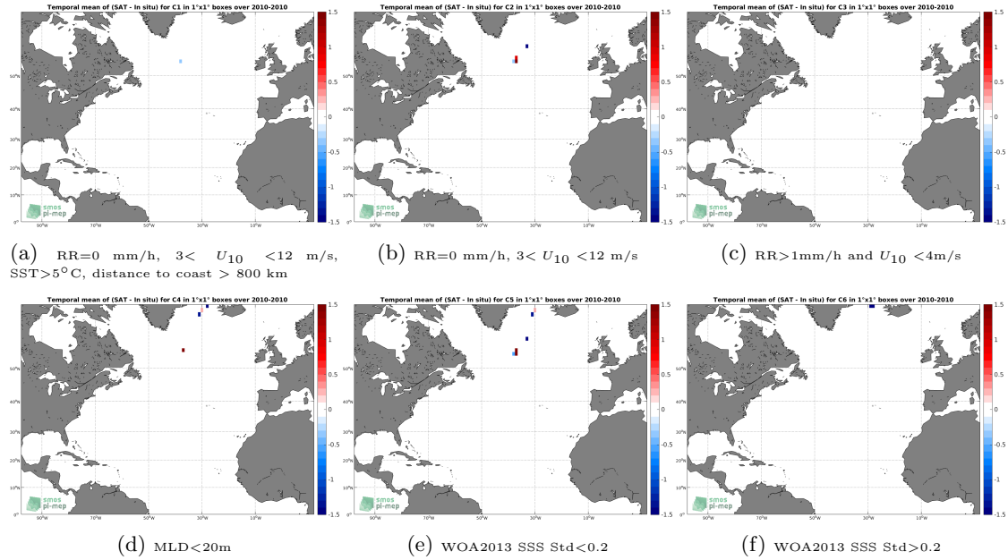
Figure 12: Temporal mean gridded over spatial boxes of size 1^{\circ}\times 1^{\circ} of \Delta\text{SSS} (SMOS SSS L2 v662 (ESA) - Sea mammals) for 6 different subdatasets corresponding to:RR=0 mm/h, 3 < U_{10} < 12 m/s, SST >5^{\circ}\text{C} , distance to coast > 800 km (a), RR=0 mm/h, 3 < U_{10} < 12 m/s (b), RR >1\text{mm/h} and U_{10} < 4\text{m/s} (c),MLD <20\text{m} (d),WOA2013 SSS Std <0.2 (e),WOA2013 SSS Std >0.2 (f).
