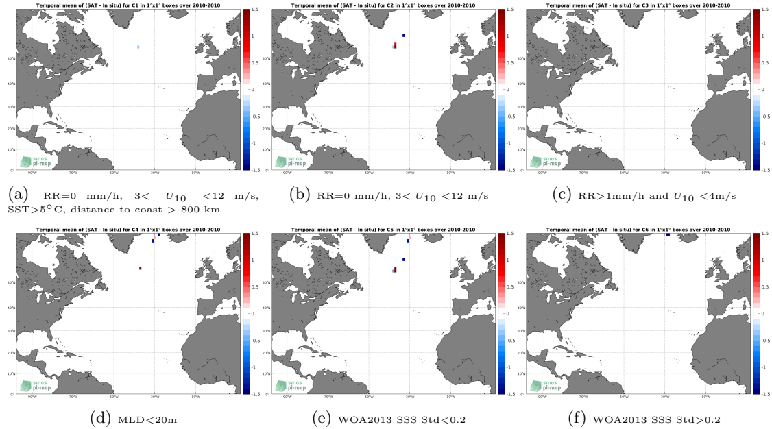
Figure 12: Temporal mean gridded over spatial boxes of size 1^{\circ}\times 1^{\circ} of \Delta\text{SSS} (SMOS SSS L2 v662 (ESA) - Sea mammals) for 6 different subdatasets corresponding to: \text{RR}=0 mm/h, 3 < U_{10} < 12 m/s, \text{SST} > 5^{\circ}\text{C} , distance to coast > 800 km (a), \text{RR}=0 mm/h, 3 < U_{10} < 12 m/s (b), \text{RR} > 1\text{mm/h} and U_{10} < 4\text{m/s} (c), \text{MLD} < 20\text{m} (d), \text{WOA2013 SSS Std} < 0.2 (e), \text{WOA2013 SSS Std} > 0.2 (f).
