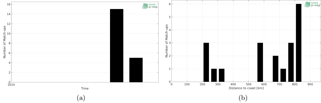
Figure 1: Number of match-ups between Sea mammals and SMOS SSS L2 v662 (ESA) SSS as a function of time (a) and as function of the distance to coast (b) over the North Atlantic Ocean Pi-MEP region and for the full satellite product period.
