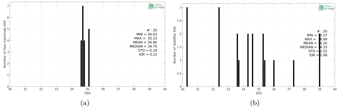
Figure 2: Histograms of SSS from Sea mammals (a) and SMOS SSS L2 v662 (ESA) (b) considering all match-up pairs per bins of 0.1 over the North Atlantic Ocean Pi-MEP region and for the full satellite product period.
