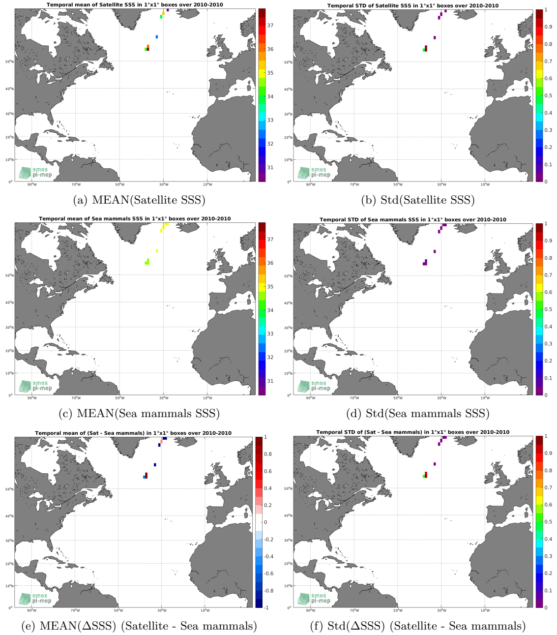
Figure 6: Temporal mean (left) and Std (right) of SSS from SMOS SSS L2 v662 (ESA) (top), Sea mammals (middle), and of \Delta SSS (Satellite - Sea mammals). Only match-up pairs are used to generate these maps.
