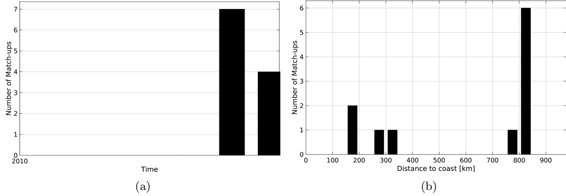
Figure 1: Number of match-ups between Sea mammals and SMOS-L2-DPGS-v662 SSS as a function of time (a) and as function of the distance to coast (b) over the North Atlantic Ocean Pi-MEP region and for the full satellite product period.
