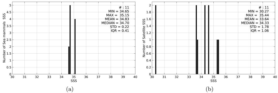
Figure 2: Histograms of SSS from Sea mammals (a) and SMOS-L2-DPGS-v662 (b) considering all match-up pairs per bins of 0.1 over the North Atlantic Ocean Pi-MEP region and for the full satellite product period.
