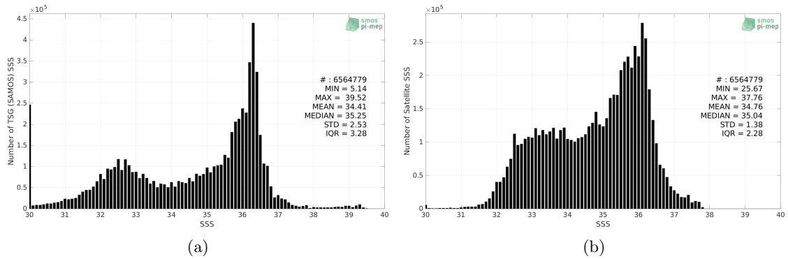
Figure 2: Histograms of SSS from TSG (SAMOS) (a) and SMAP SSS L4 OI v1 - 7 Days (IPRC) (b) considering all match-up pairs per bins of 0.1 over the North Atlantic Ocean Pi-MEP region and for the full satellite product period.
