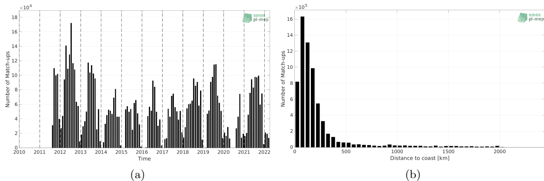
Figure 1: Number of match-ups between TSG (SAMOS) and SMAP SSS L4 OI v1 - 7 Days (IPRC) SSS as a function of time (a) and as function of the distance to coast (b) over the North Atlantic Ocean Pi-MEP region and for the full satellite product period.
