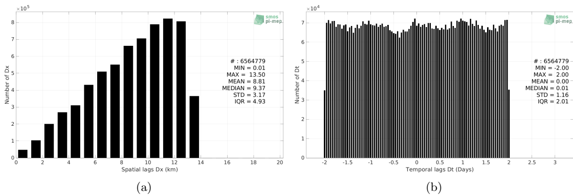
Figure 5: Histograms of the spatial (a) and temporal (b) lags between the location/time of the TSG (SAMOS) measurement and the date of the corresponding SMAP SSS L4 OI v1 - 7 Days (IPRC) SSS pixel.
