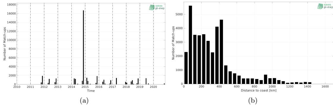
Figure 1: Number of match-ups between TSG (Polarstern) and SMAP SSS L4 OI v1 - 7 Days (IPRC) SSS as a function of time (a) and as function of the distance to coast (b) over the North Atlantic Ocean Pi-MEP region and for the full satellite product period.
