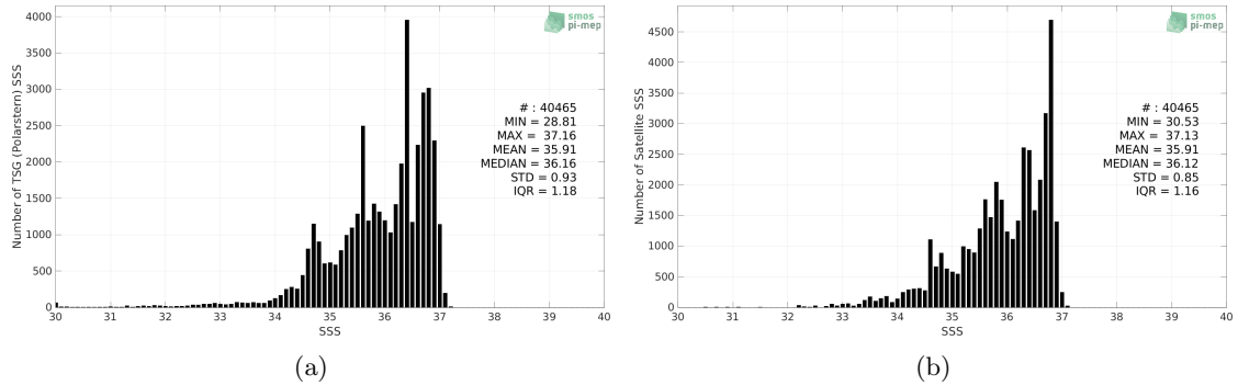
Figure 2: Histograms of SSS from TSG (Polarstern) (a) and SMAP SSS L4 OI v1 - 7 Days (IPRC) (b) considering all match-up pairs per bins of 0.1 over the North Atlantic Ocean Pi-MEP region and for the full satellite product period.
