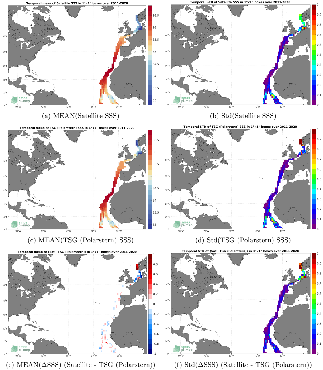
Figure 6: Temporal mean (left) and Std (right) of SSS from SMAP SSS L4 OI v1 - 7 Days (IPRC) (top), TSG (Polarstern) (middle), and of \Delta SSS (Satellite - TSG (Polarstern)). Only match-up pairs are used to generate these maps.
