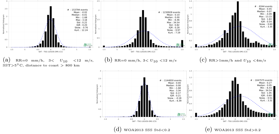
Figure 13: Normalized histogram of \Delta\text{SSS} (SMAP SSS L4 OI v1 - 7 Days (IPRC) - TSG (LEGOS-DM)) for 5 different subdatasets corresponding to: RR=0 mm/h, 3 < U_{10} < 12 m/s, SST>5°C, distance to coast > 800 km (a), RR=0 mm/h, 3 < U_{10} < 12 m/s (b), RR>1mm/h and U_{10} < 4 m/s (c), WOA2013 SSS Std<0.2 (d), WOA2013 SSS Std>0.2 (e).
