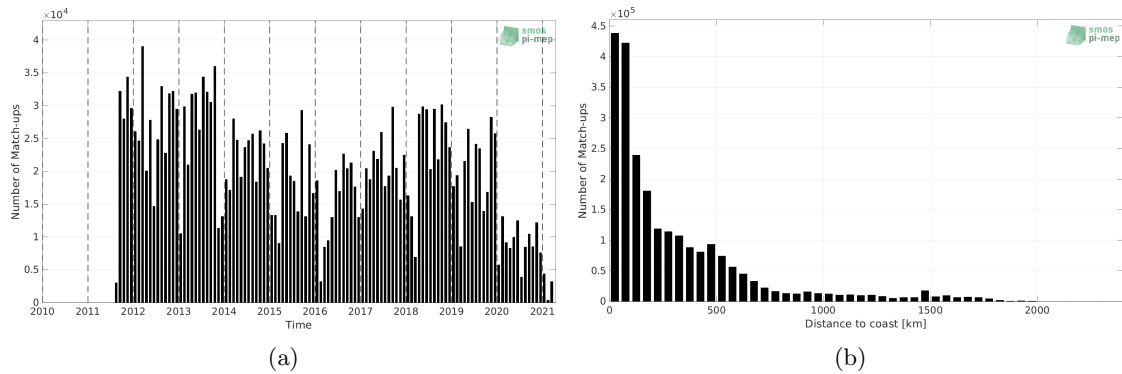
Figure 1: Number of match-ups between TSG (LEGOS-DM) and SMAP SSS L4 OI v1 - 7 Days (IPRC) SSS as a function of time (a) and as function of the distance to coast (b) over the North Atlantic Ocean Pi-MEP region and for the full satellite product period.
