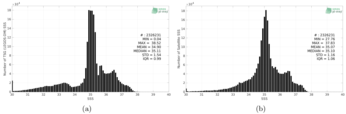
Figure 2: Histograms of SSS from TSG (LEGOS-DM) (a) and SMAP SSS L4 OI v1 - 7 Days (IPRC) (b) considering all match-up pairs per bins of 0.1 over the North Atlantic Ocean Pi-MEP region and for the full satellite product period.
