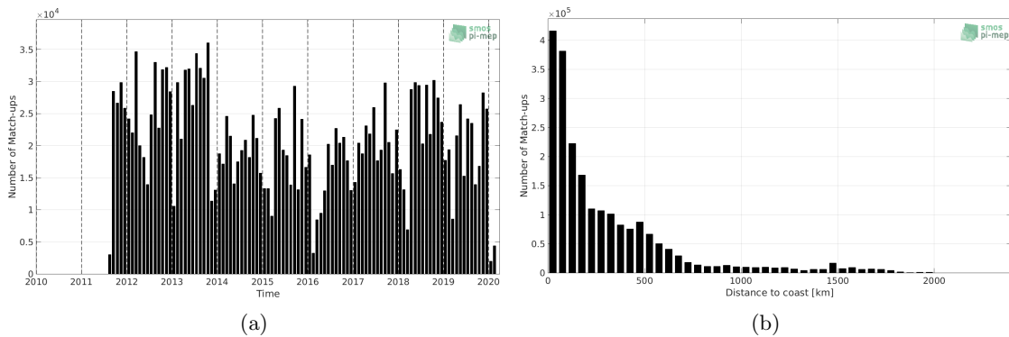
Figure 1: Number of match-ups between TSG (LEGOS-DM) and SMAP SSS L4 OI v1 - 7day (IPRC) SSS as a function of time (a) and as function of the distance to coast (b) over the North Atlantic Ocean Pi-MEP region and for the full satellite product period.
