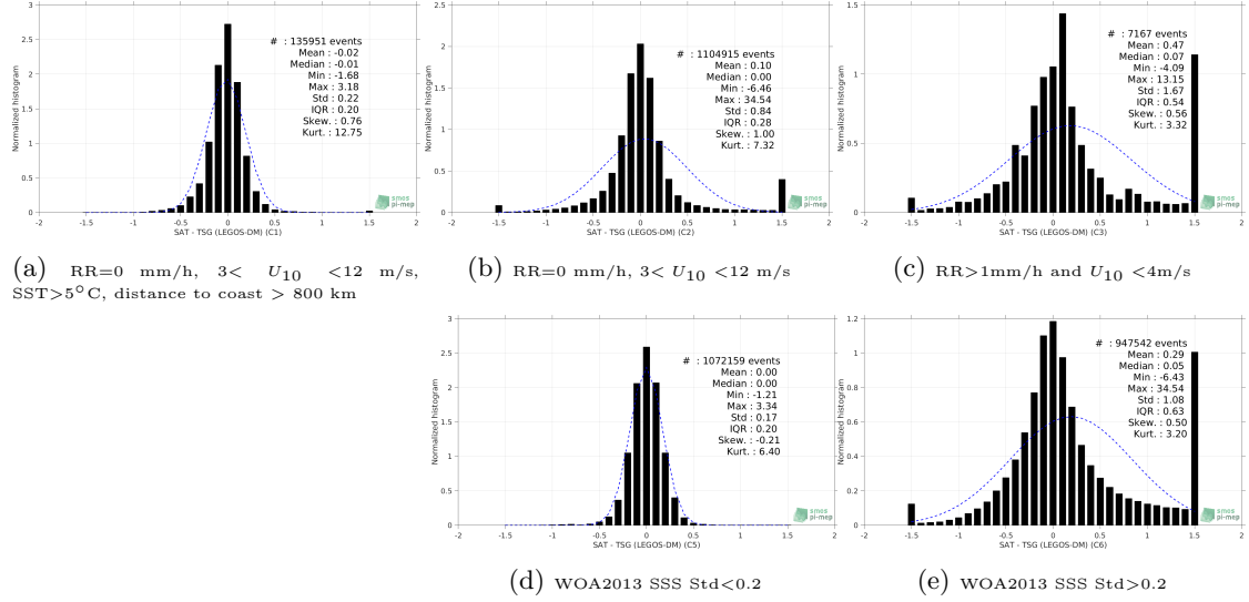
Figure 13: Normalized histogram of \Delta SSS (SMAP SSS L4 OI v1 - 7day (IPRC) - TSG (LEGOS-DM)) for 5 different subdatasets corresponding to: RR=0 mm/h, 3 < U_{10} < 12 m/s, SST > 5°C, distance to coast > 800 km (a), RR=0 mm/h, 3 < U_{10} < 12 m/s (b), RR > 1mm/h and U_{10} < 4 m/s (c), WOA2013 SSS Std < 0.2 (d), WOA2013 SSS Std > 0.2 (e).
