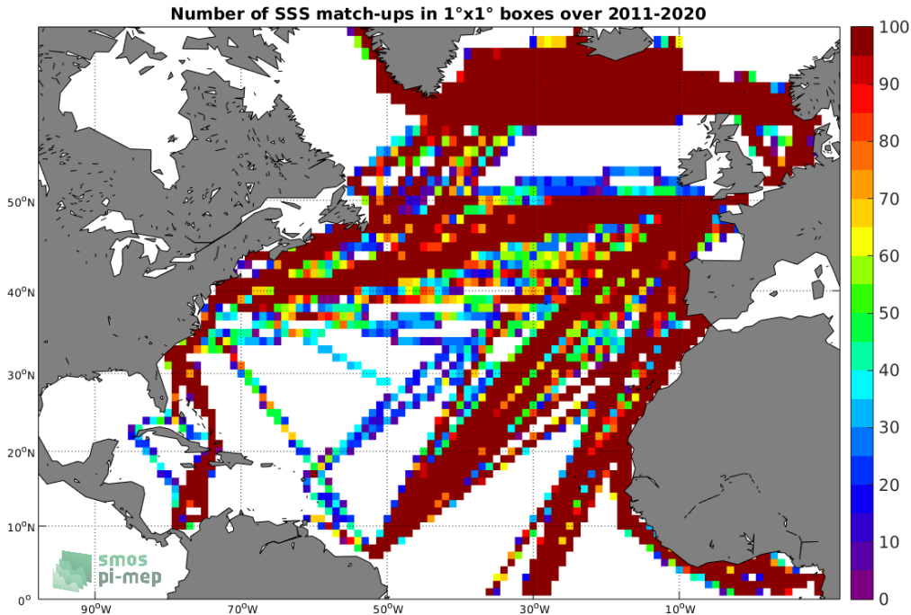
Figure 4: Number of SSS match-ups between TSG (LEGOS-DM) SSS and the SMAP SSS L4 OI v1 - 7day (IPRC) SSS product for the North Atlantic Ocean Pi-MEP region over 1°x1° boxes and for the full satellite product period.
