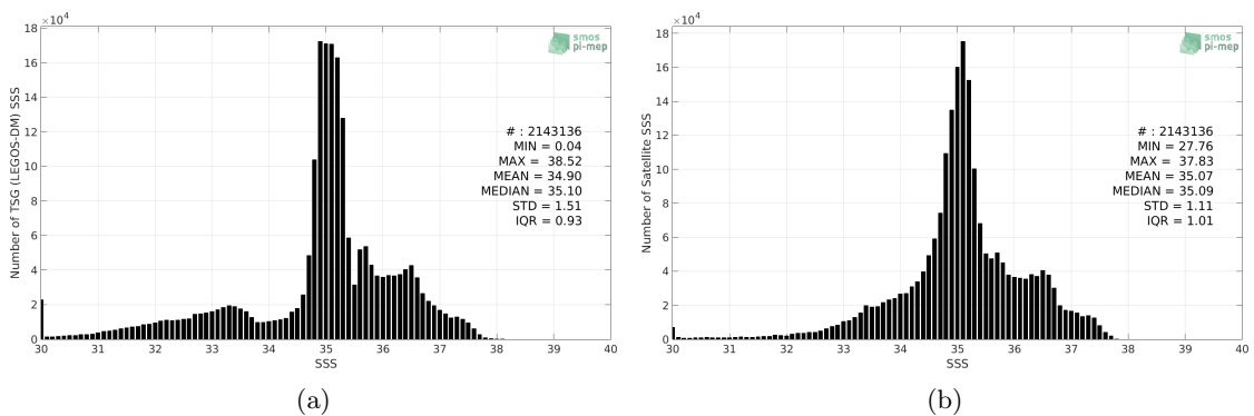
Figure 2: Histograms of SSS from TSG (LEGOS-DM) (a) and SMAP SSS L4 OI v1 - 7day (IPRC) (b) considering all match-up pairs per bins of 0.1 over the North Atlantic Ocean Pi-MEP region and for the full satellite product period.
