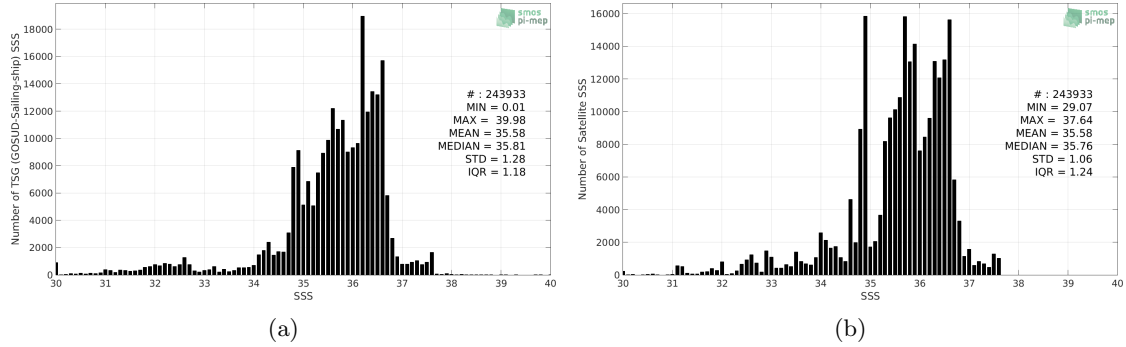
Figure 2: Histograms of SSS from TSG (GOSUD-Sailing-ship) (a) and SMAP SSS L4 OI v1 - 7 Days (IPRC) (b) considering all match-up pairs per bins of 0.1 over the North Atlantic Ocean Pi-MEP region and for the full satellite product period.
