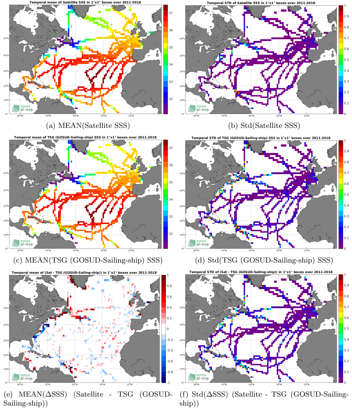
Figure 6: Temporal mean (left) and Std (right) of SSS from SMAP SSS L4 OI v1 - 7day (IPRC) (top), TSG (GOSUD-Sailing-ship) (middle), and of \Delta SSS (Satellite - TSG (GOSUD-Sailing-ship)). Only match-up pairs are used to generate these maps.
