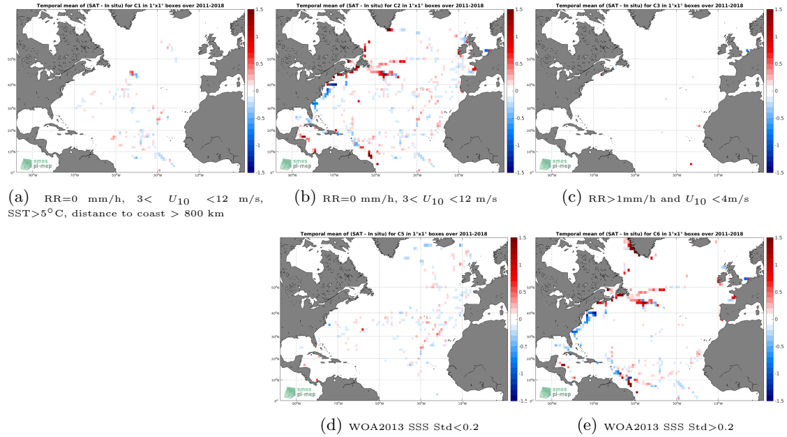
Figure 12: Temporal mean gridded over spatial boxes of size 1^\circ \times 1^\circ of \Delta SSS (SMAP SSS L4 OI v1 - 7day (IPRC) - TSG (GOSUD-Sailing-ship)) for 5 different subdatasets corresponding to: RR=0 mm/h, 3 < U_{10} < 12 m/s, SST >5^\circ\text{C} , distance to coast > 800 km (a), RR=0 mm/h, 3 < U_{10} < 12 m/s (b), RR >1 mm/h and U_{10} < 4 m/s (c), WOA2013 SSS Std <0.2 (d), WOA2013 SSS Std >0.2 (e).
