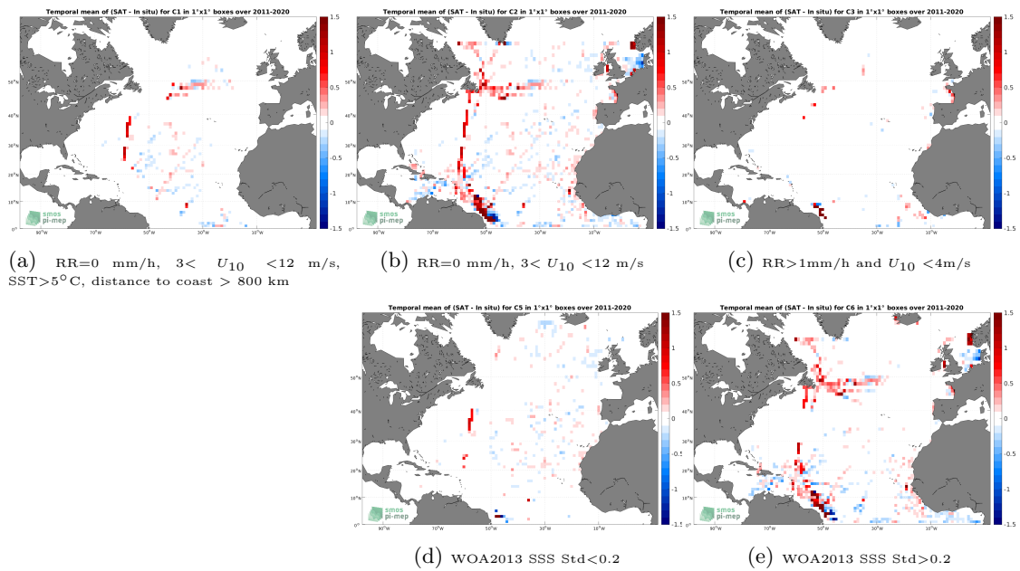
Figure 12: Temporal mean gridded over spatial boxes of size 1^\circ \times 1^\circ of \Delta\text{SSS} (SMAP SSS L4 OI v1 - 7 Days (IPRC) - TSG (GOSUD-Research-vessel)) for 5 different subdatasets corresponding to:RR=0 mm/h, 3 < U_{10} < 12 m/s, SST>5°C, distance to coast > 800 km (a), RR=0 mm/h, 3 < U_{10} < 12 m/s (b), RR>1mm/h and U_{10} < 4 m/s (c), WOA2013 SSS Std<0.2 (d), WOA2013 SSS Std>0.2 (e).
