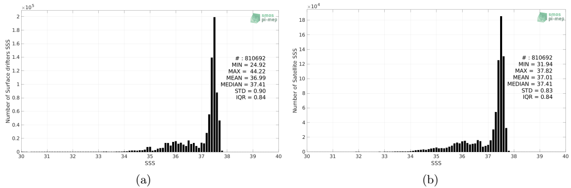
Figure 2: Histograms of SSS from Surface drifters (a) and SMAP SSS L4 OI v1 - 7 Days (IPRC) (b) considering all match-up pairs per bins of 0.1 over the North Atlantic Ocean Pi-MEP region and for the full satellite product period.
