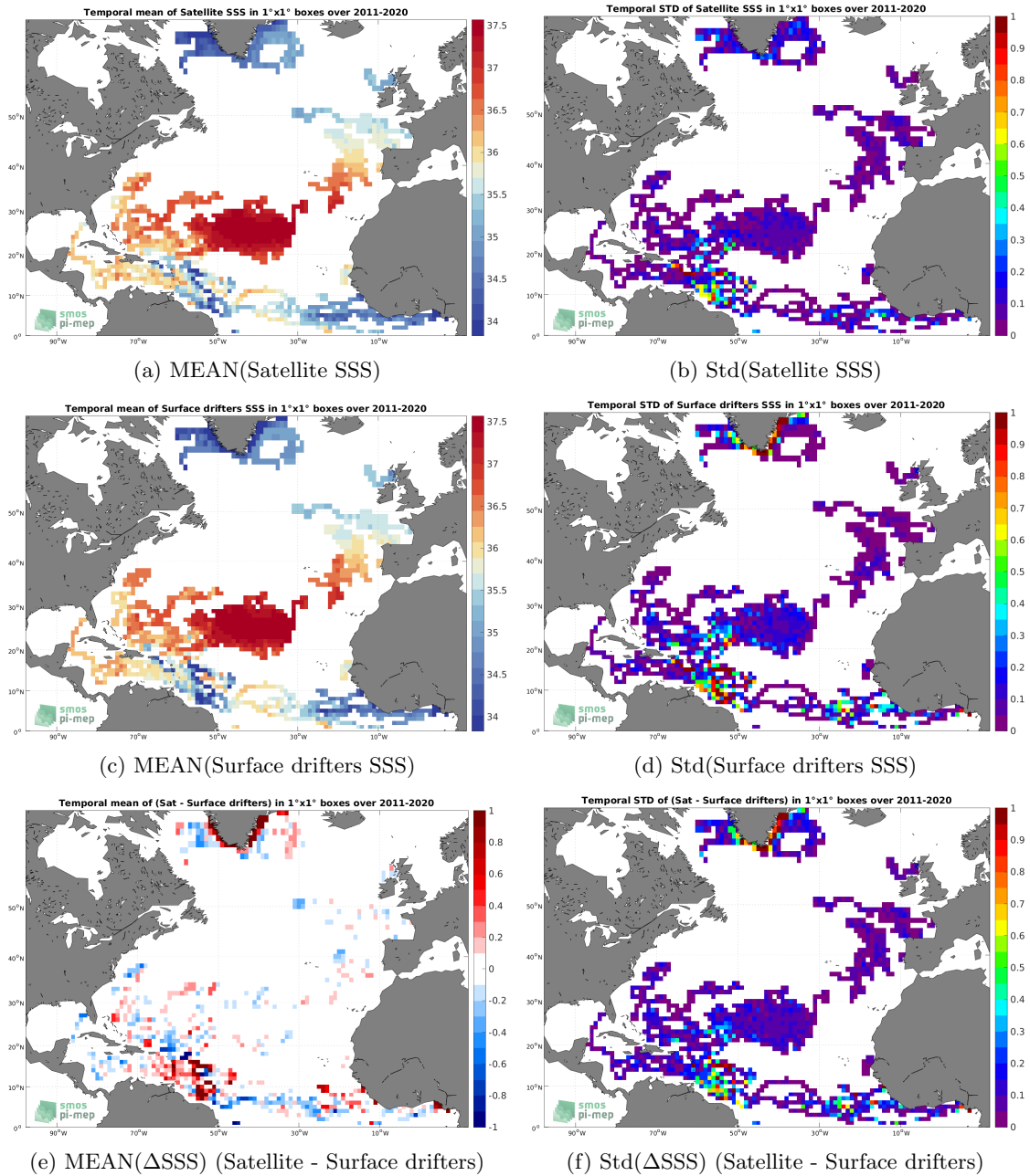
Figure 5: Temporal mean (left) and Std (right) of SSS from SMAP SSS L4 OI v1 - 7 Days (IPRC) (top), Surface drifters (middle), and of \Delta SSS (Satellite - Surface drifters). Only match-up pairs are used to generate these maps.
