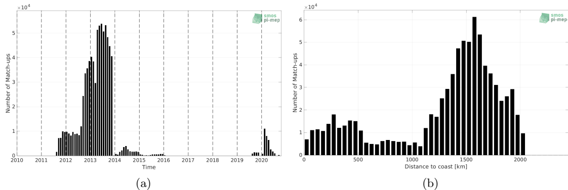
Figure 1: Number of match-ups between Surface drifters and SMAP SSS L4 OI v1 - 7 Days (IPRC) SSS as a function of time (a) and as function of the distance to coast (b) over the North Atlantic Ocean Pi-MEP region and for the full satellite product period.
