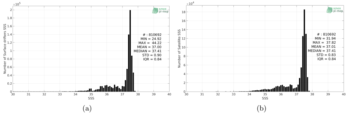
Figure 2: Histograms of SSS from Surface drifters (a) and SMAP SSS L4 OI v1 - 7day (IPRC) (b) considering all match-up pairs per bins of 0.1 over the North Atlantic Ocean Pi-MEP region and for the full satellite product period.
