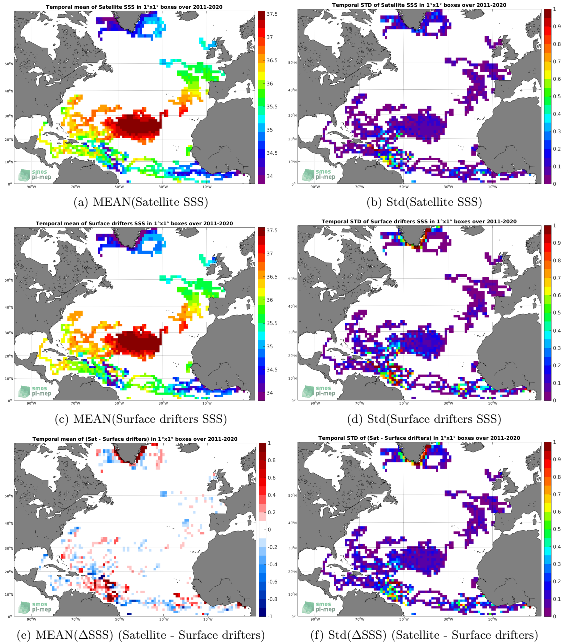
Figure 5: Temporal mean (left) and Std (right) of SSS from SMAP SSS L4 OI v1 - 7day (IPRC) (top), Surface drifters (middle), and of \Delta SSS (Satellite - Surface drifters). Only match-up pairs are used to generate these maps.
