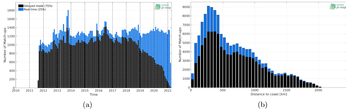
Figure 1: Number of match-ups between Argo and SMAP SSS L4 OI v1 - 7 Days (IPRC) SSS as a function of time (a) and as function of the distance to coast (b) over the North Atlantic Ocean Pi-MEP region and for the full satellite product period.
