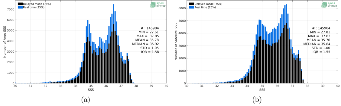
Figure 2: Histograms of SSS from Argo (a) and SMAP SSS L4 OI v1 - 7 Days (IPRC) (b) considering all match-up pairs per bins of 0.1 over the North Atlantic Ocean Pi-MEP region and for the full satellite product period.
