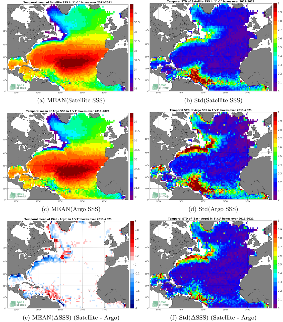
Figure 6: Temporal mean (left) and Std (right) of SSS from SMAP SSS L4 OI v1 - 7 Days (IPRC) (top), Argo (middle), and of \Delta SSS (Satellite - Argo). Only match-up pairs are used to generate these maps.
