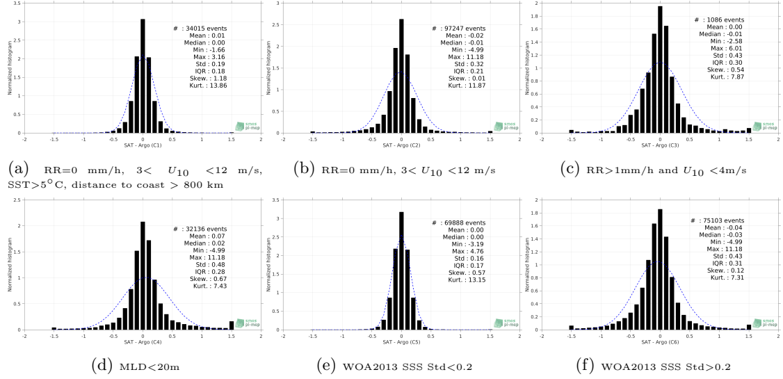
Figure 13: Normalized histogram of \Delta SSS (SMAP SSS L4 OI v1 - 7 Days (IPRC) - Argo) for 6 different subdatasets corresponding to: RR=0 mm/h, 3 < U_{10} < 12 m/s, SST>5°C, distance to coast > 800 km (a), RR=0 mm/h, 3 < U_{10} < 12 m/s (b), RR>1mm/h and U_{10} < 4 m/s (c), MLD<20m (d), WOA2013 SSS Std<0.2 (e), WOA2013 SSS Std>0.2 (f).
